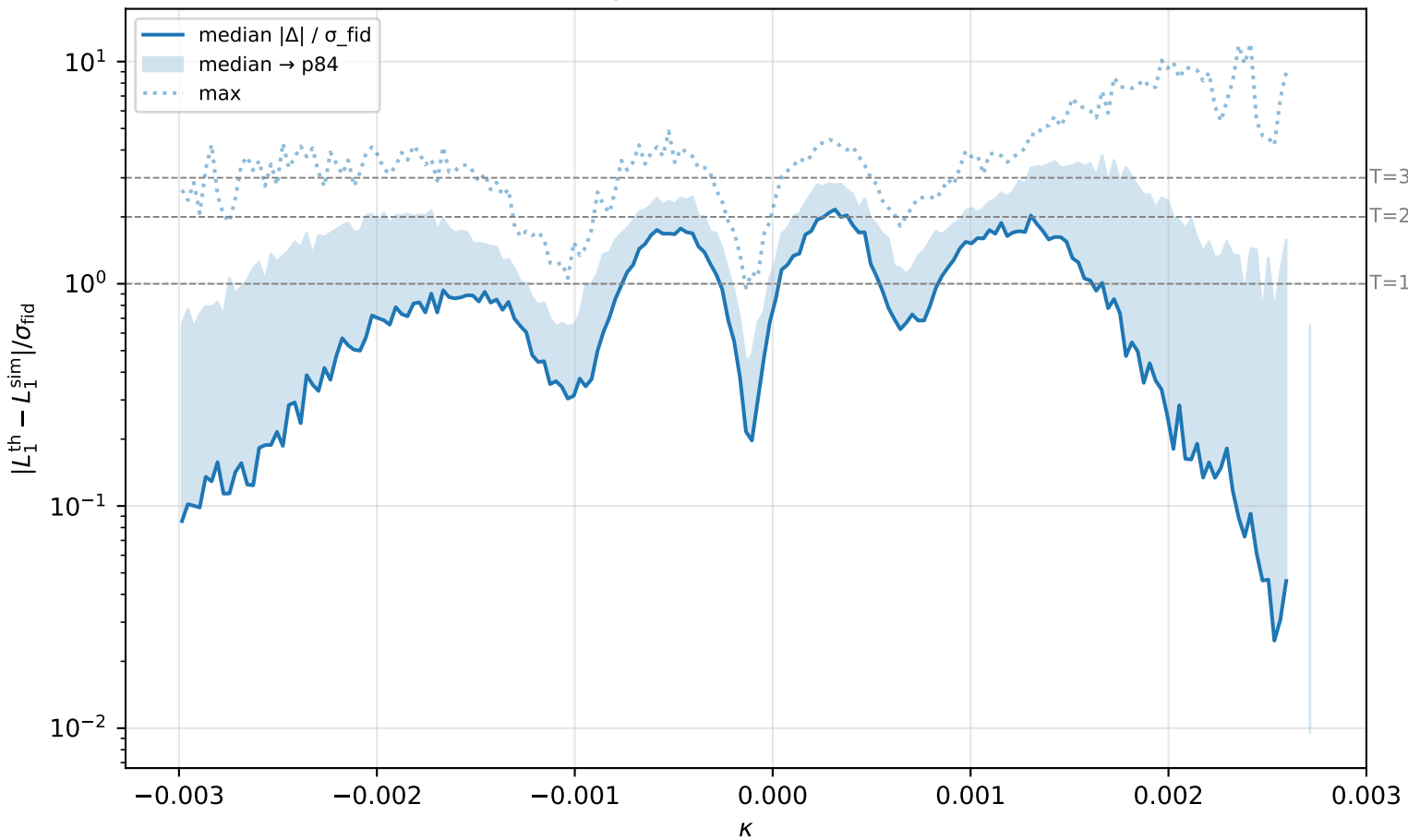
L1 residual per-cosmo distribution, \theta=20'
