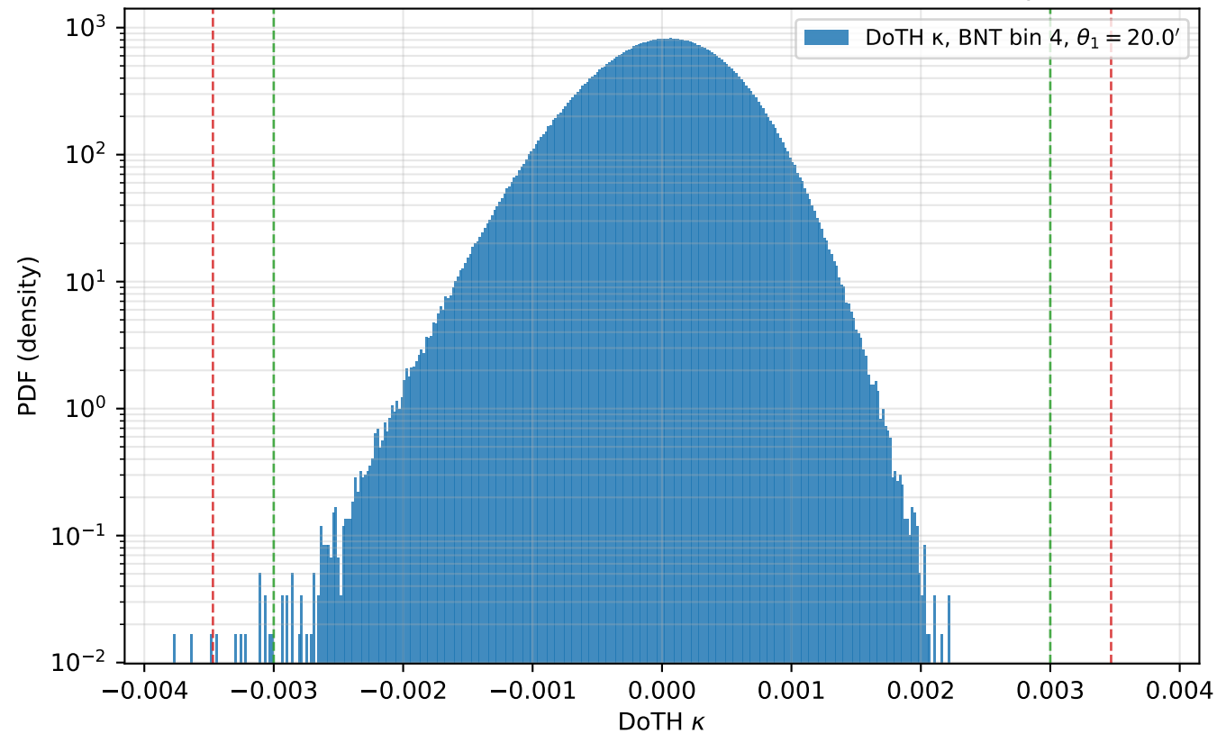
BNT bin 4 DoTH PDF — \sigma=4.957\text{e-}04 , \pm 0.003 envelope
