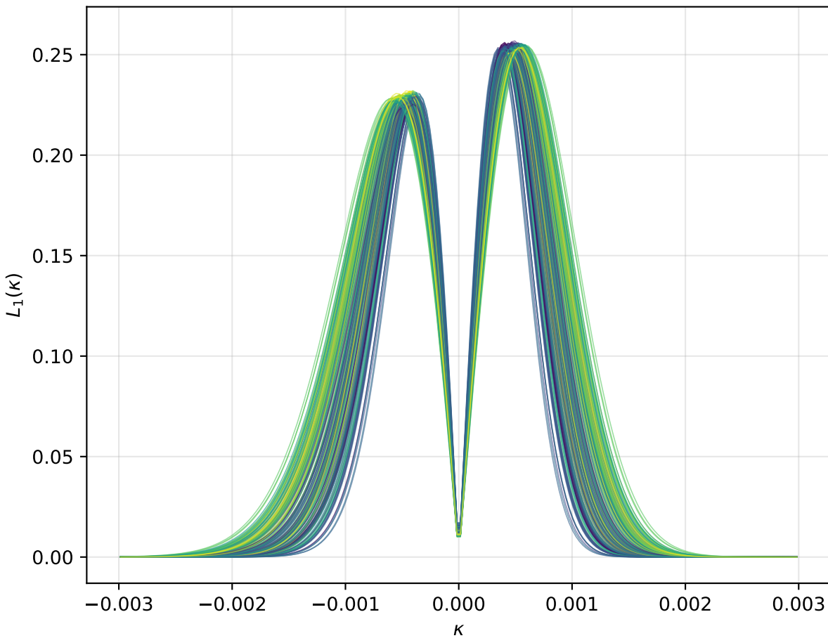
Theory L_1 (per cosmology), \theta=20.0'
