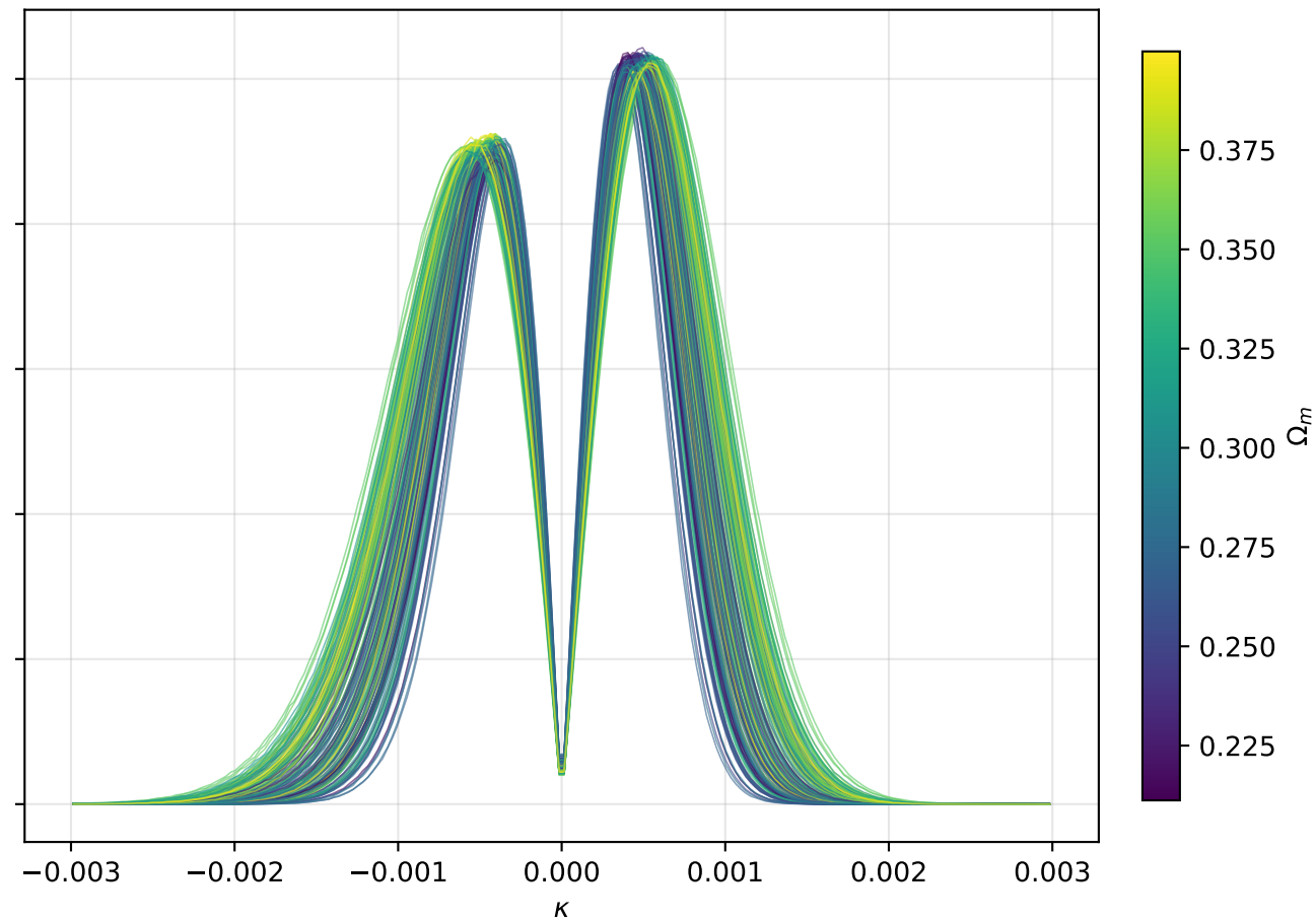
Sim L_1 mean (per cosmology, over 7 perms), \theta=20.0'
