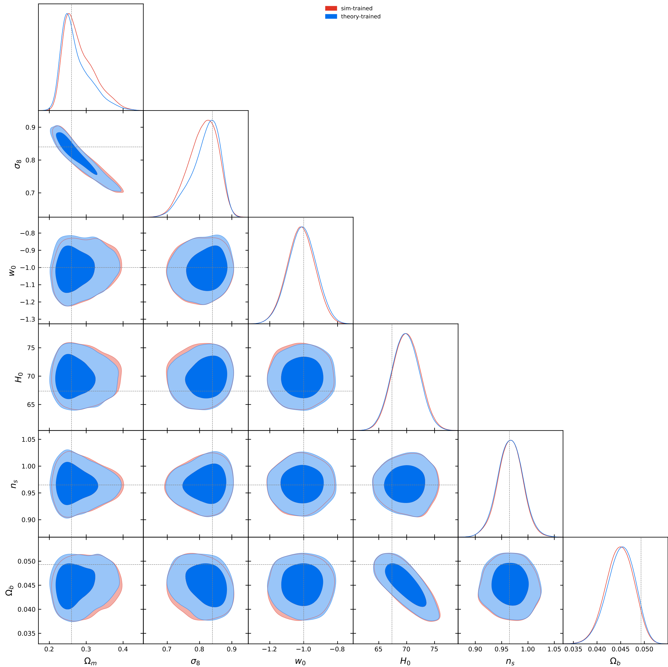
L1 NPE contours [bnt4]: sim vs theory, theta20, cut=aminm0p0003_amaxp0p0003
