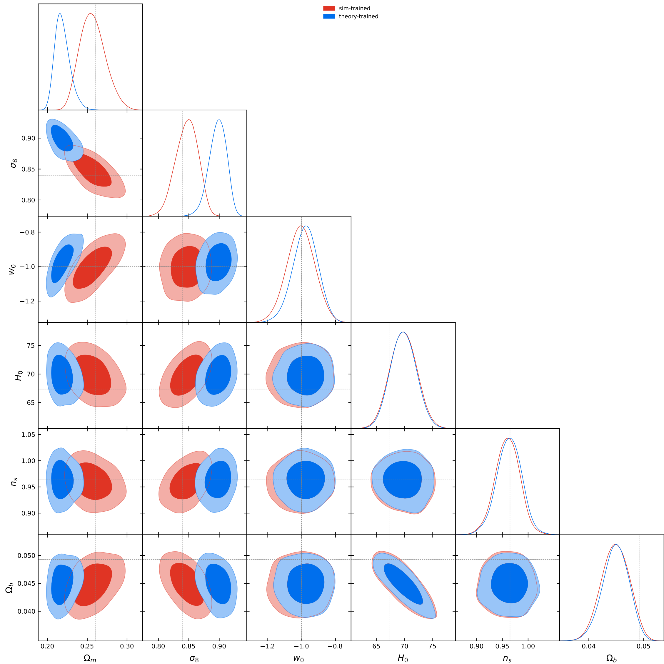
L1 NPE contours [bnt4]: sim vs theory, theta20, cut=aminm0p0005_amaxp0p0005
