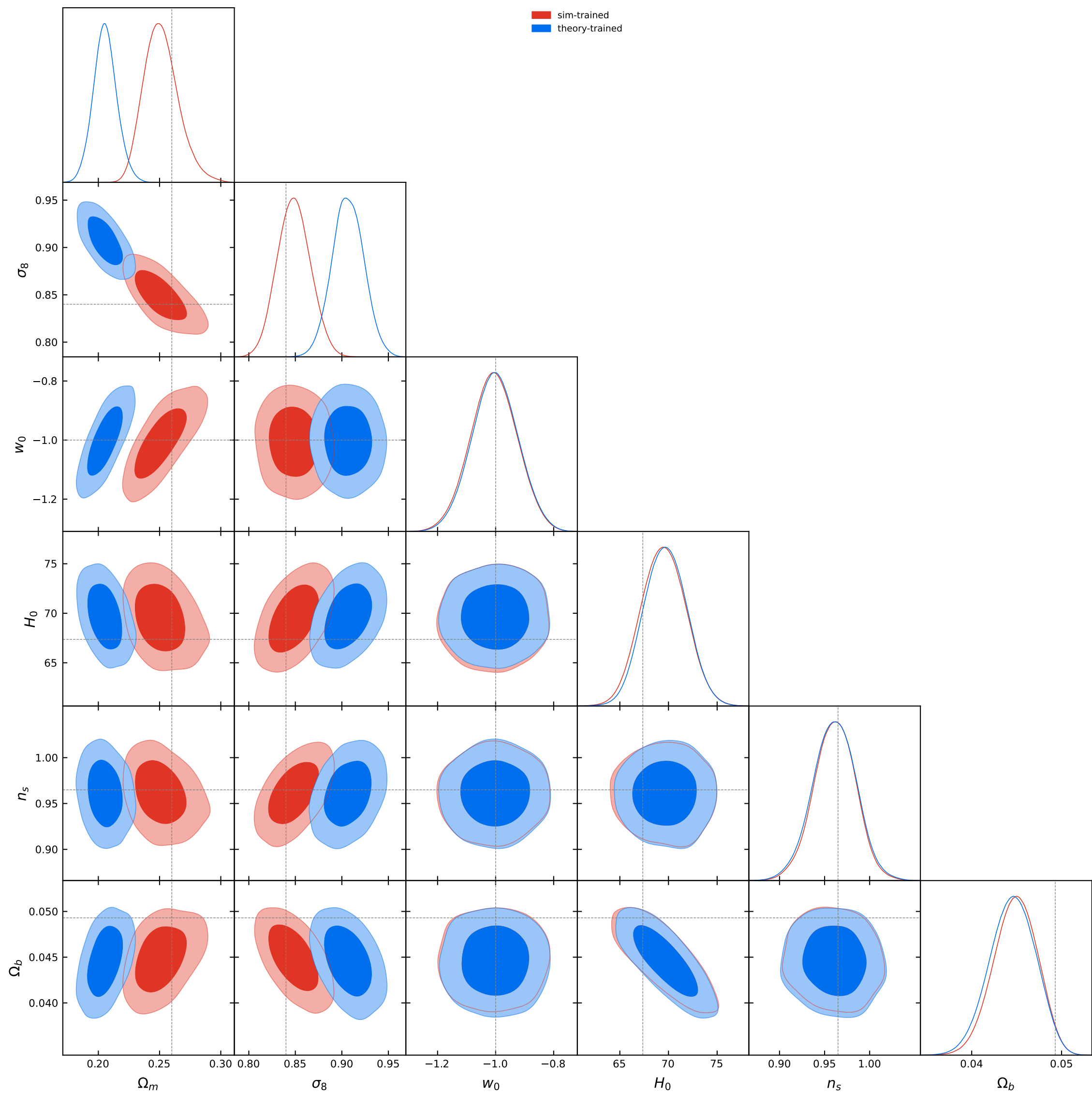
L1 NPE contours [bnt4]: sim vs theory, theta20, cut=full
