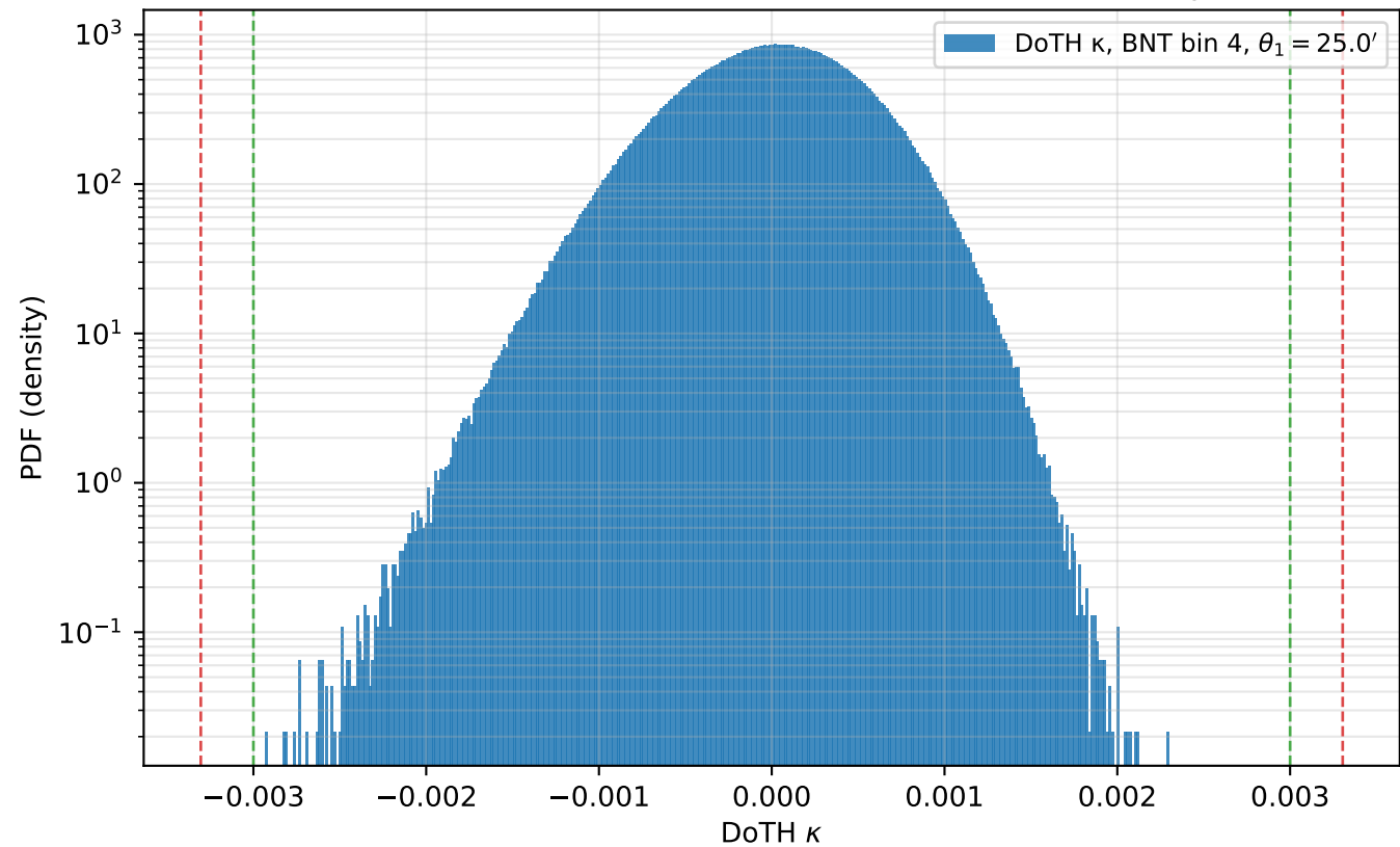
BNT bin 4 DoTH PDF — \sigma=4.721\text{e-}04 , \pm 0.003 envelope
