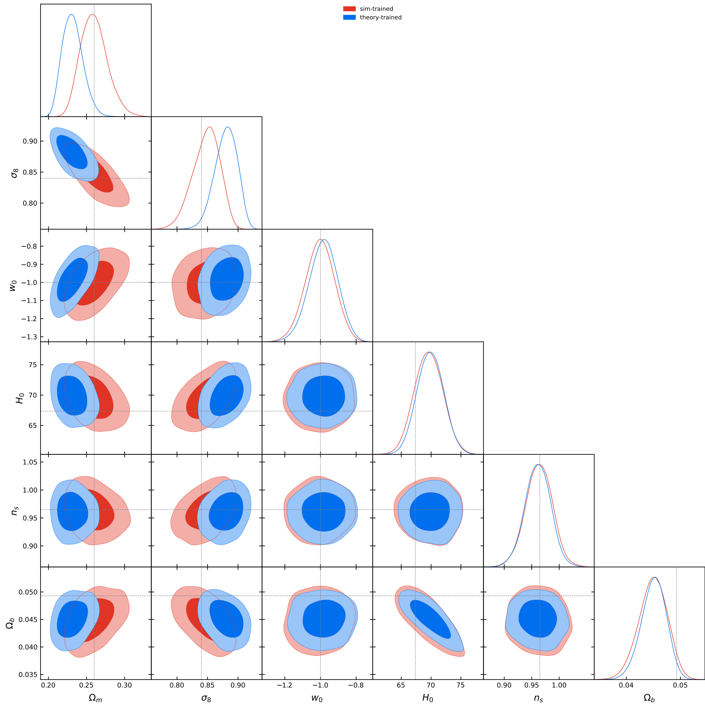
L1 NPE contours [bnt4]: sim vs theory, theta25, cut=aminm0p0005_amaxp0p0005
