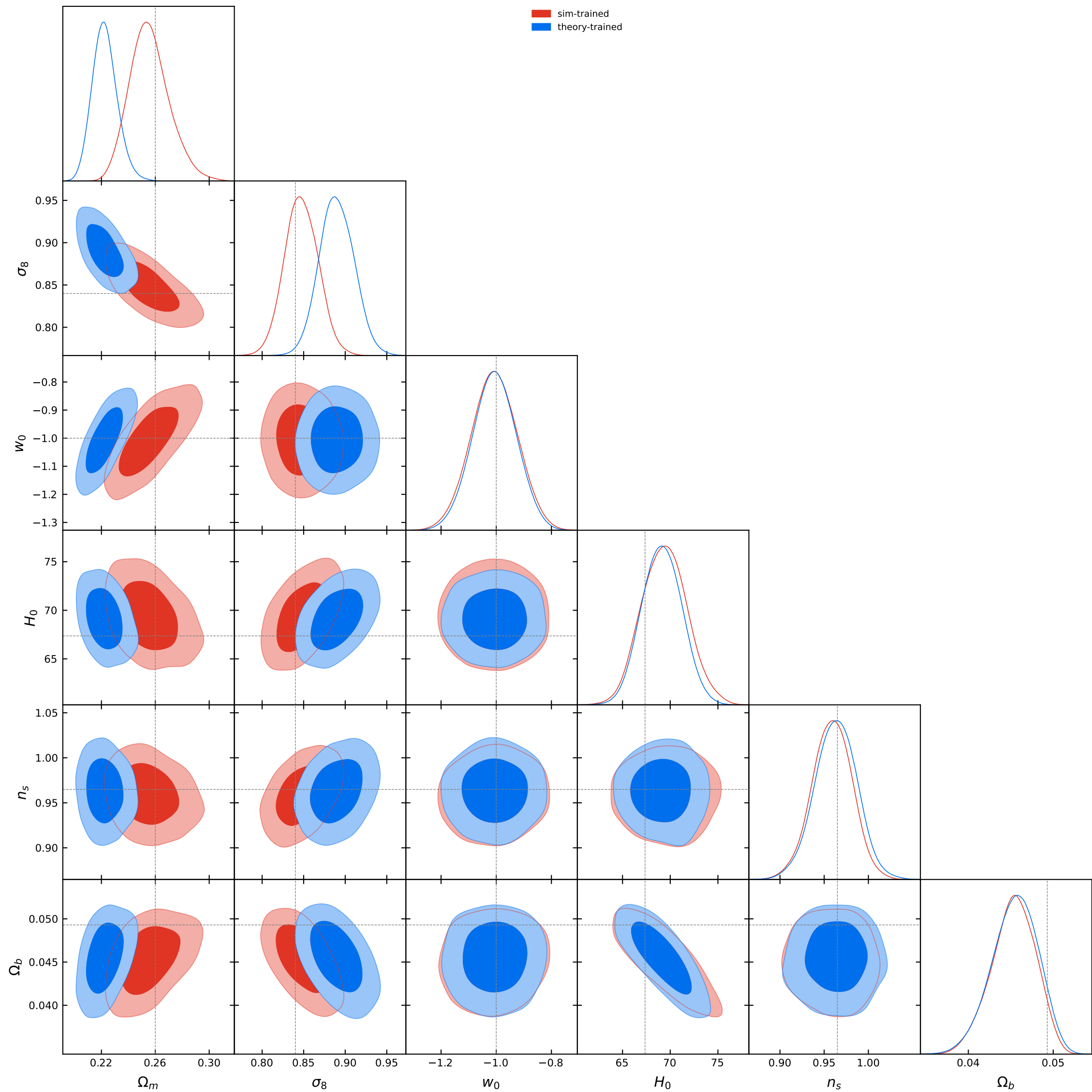
L1 NPE contours [bnt4]: sim vs theory, theta25, cut=full
