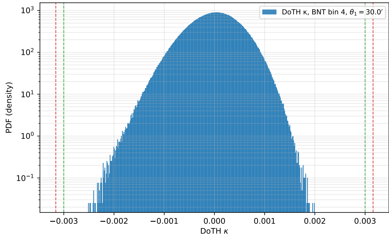
BNT bin 4 DoTH PDF — \sigma=4.513\text{e-}04 , \pm 0.003 envelope
