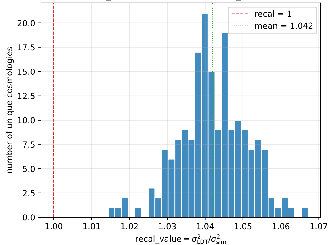
recal_value distribution — bnt4_theta30
