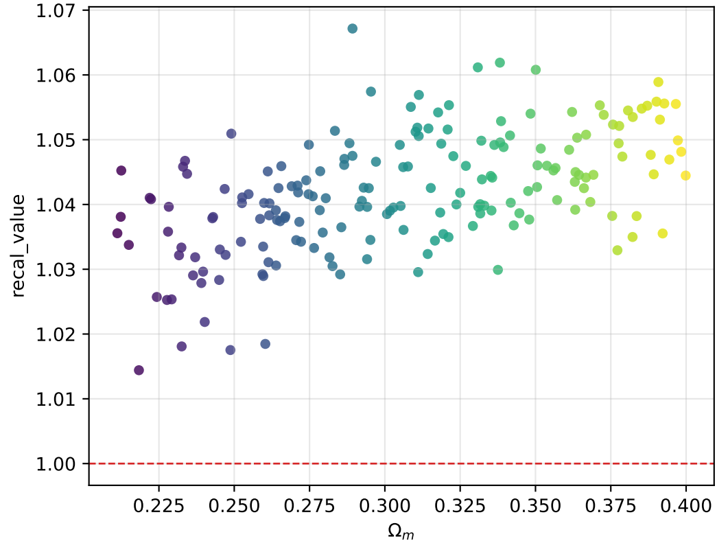
recal_value vs \Omega_m
