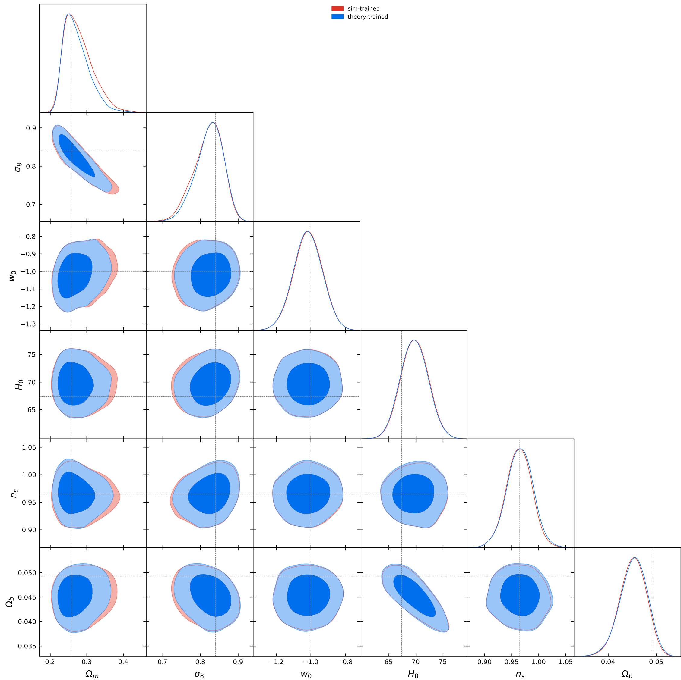
L1 NPE contours [bnt4]: sim vs theory, theta30, cut=aminm0p0003_amaxp0p0003
