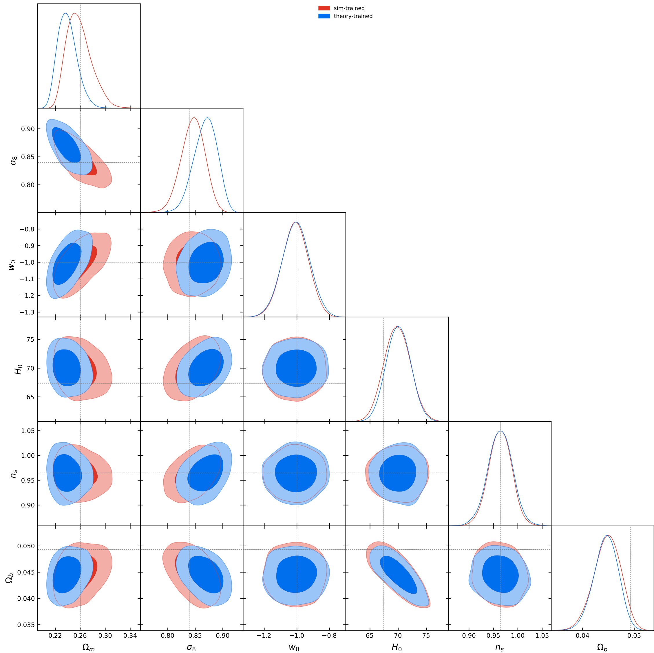
L1 NPE contours [bnt4]: sim vs theory, theta30, cut=aminm0p0005_amaxp0p0009
