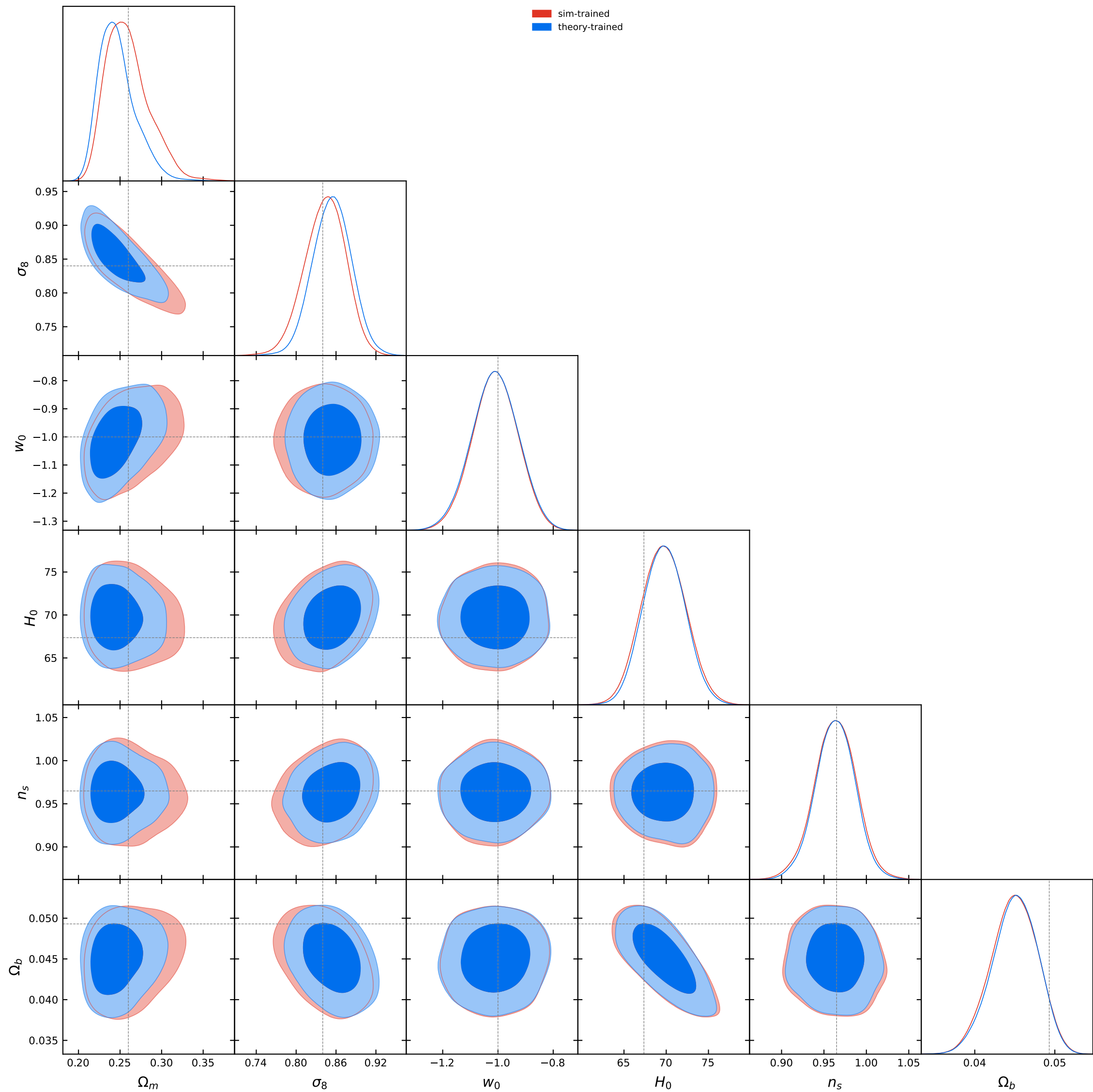
L1 NPE contours [bnt4]: sim vs theory, theta30, cut=aminm0p0006_amaxp0p0003
