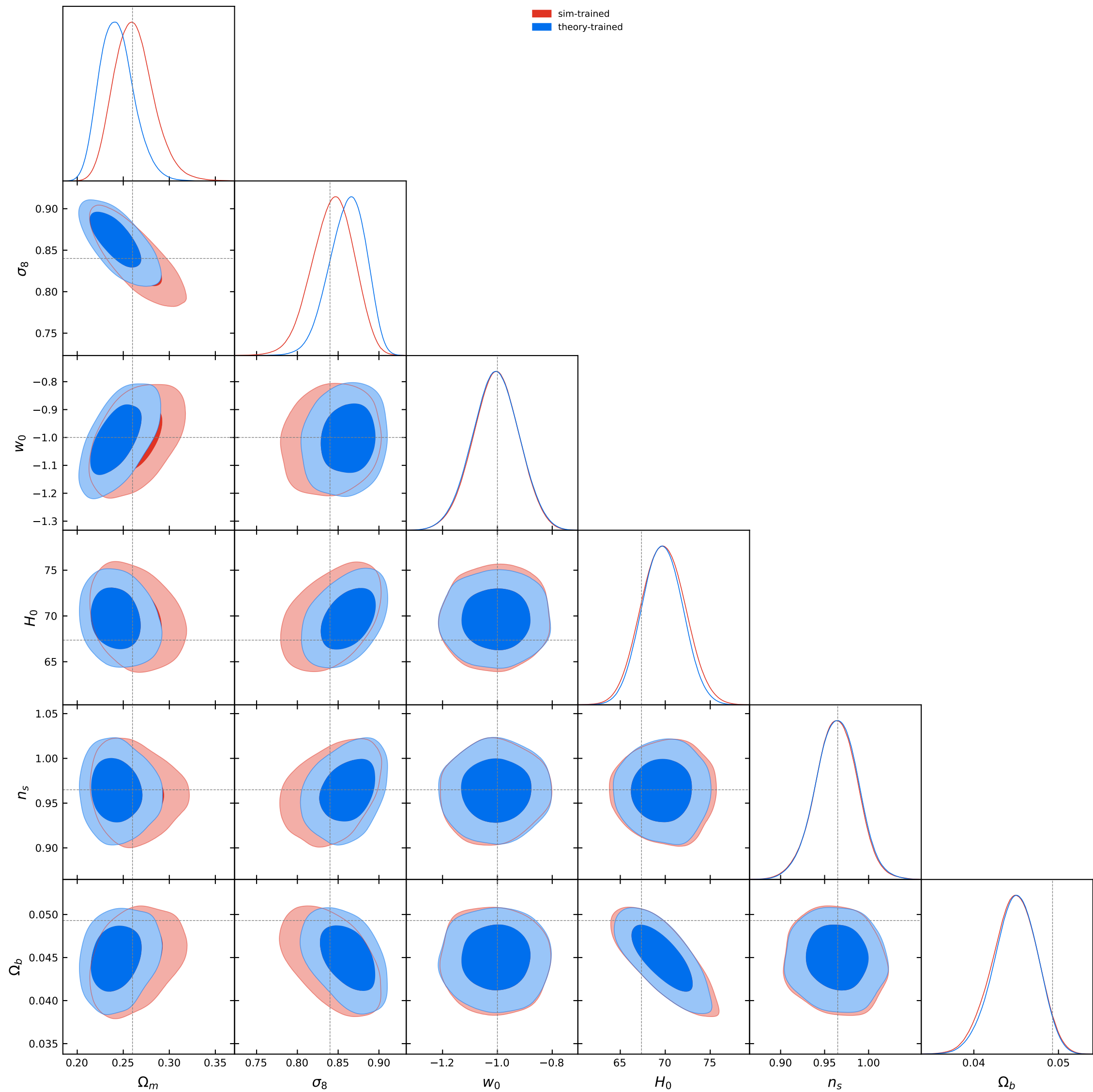
L1 NPE contours [bnt4]: sim vs theory, theta30, cut=aminm0p0009_amaxp0p0005
