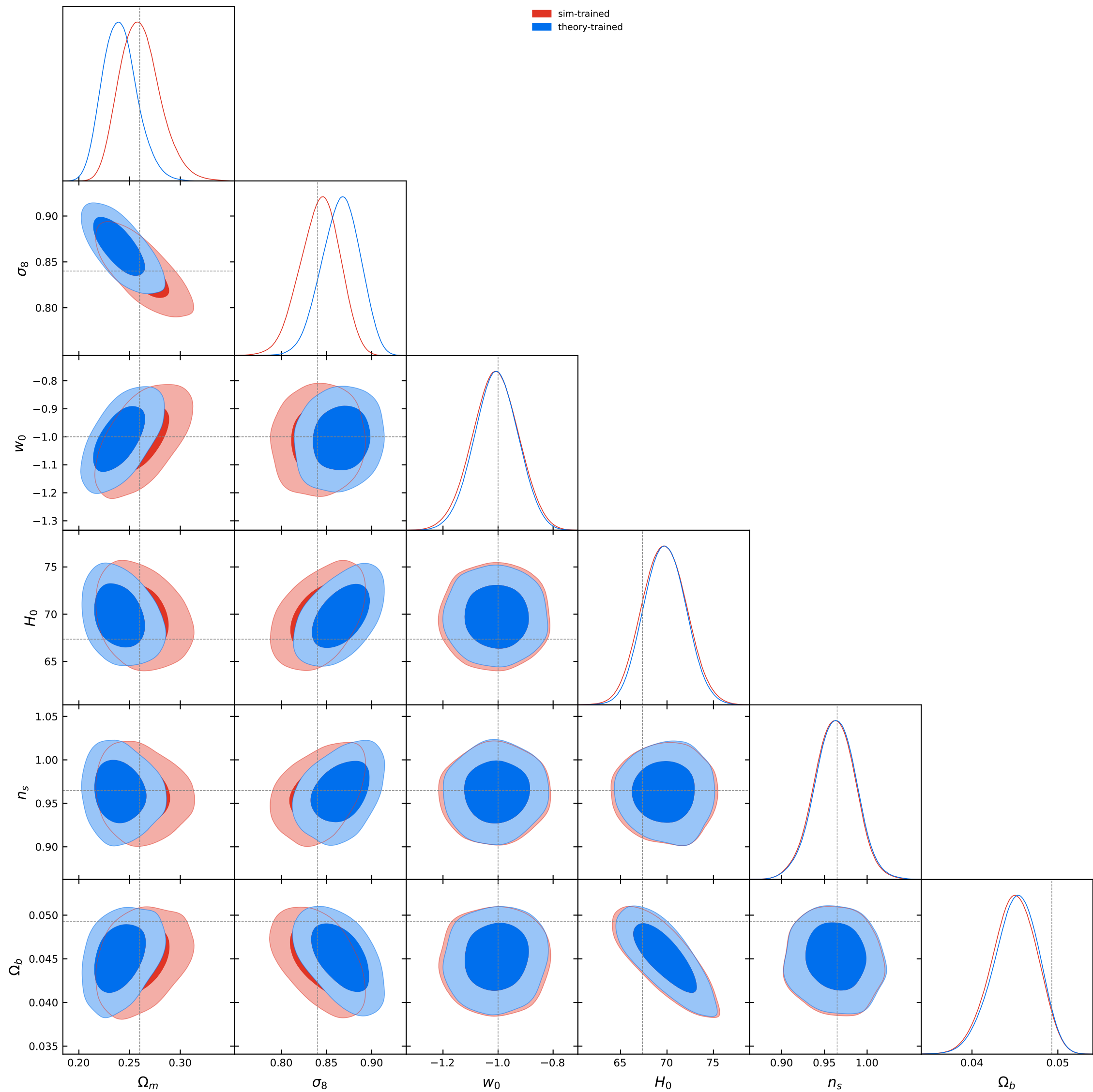
L1 NPE contours [bnt4]: sim vs theory, theta30, cut=aminm0p0009_amaxp0p0009
