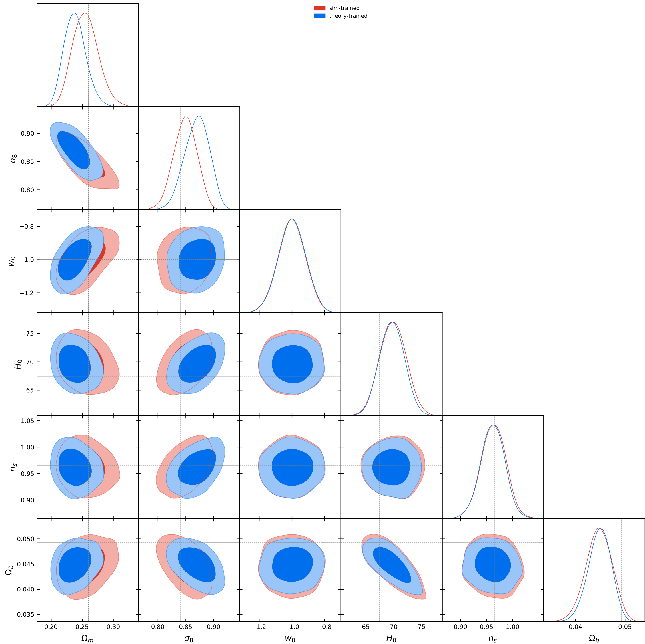
L1 NPE contours [bnt4]: sim vs theory, theta30, cut=aminm0p0015_amaxp0p0009
