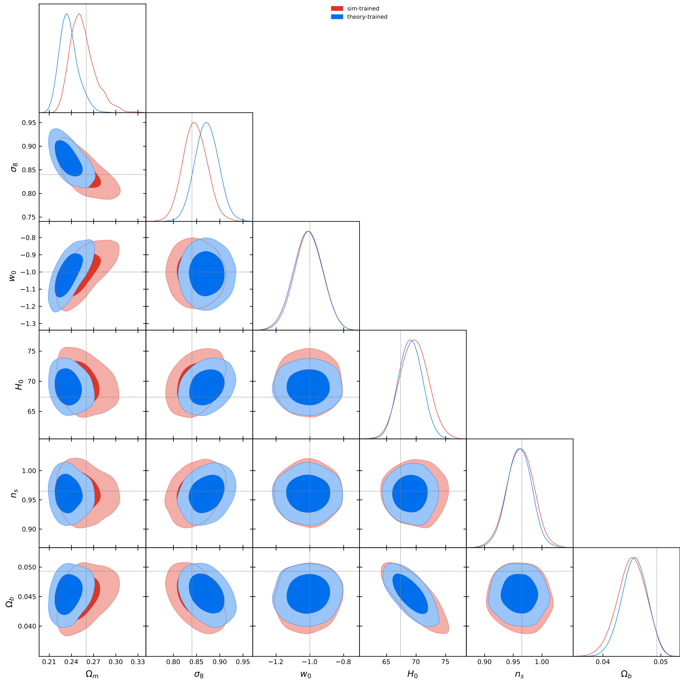
L1 NPE contours [bnt4]: sim vs theory, theta30, cut=aminm0p0024_amaxp0p0024
