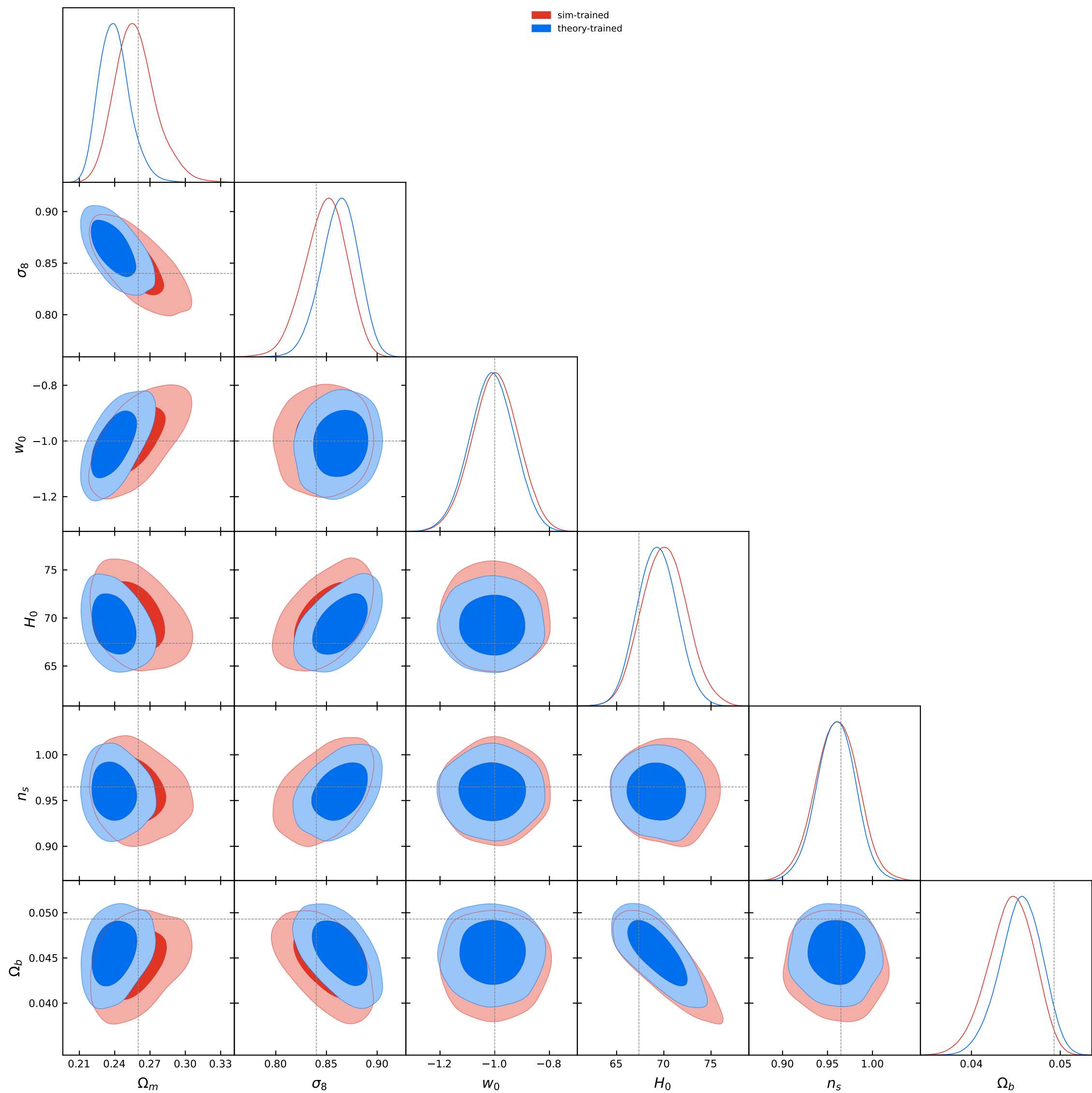
L1 NPE contours [bnt4]: sim vs theory, theta30, cut=aminm0p002_amaxp0p0015
