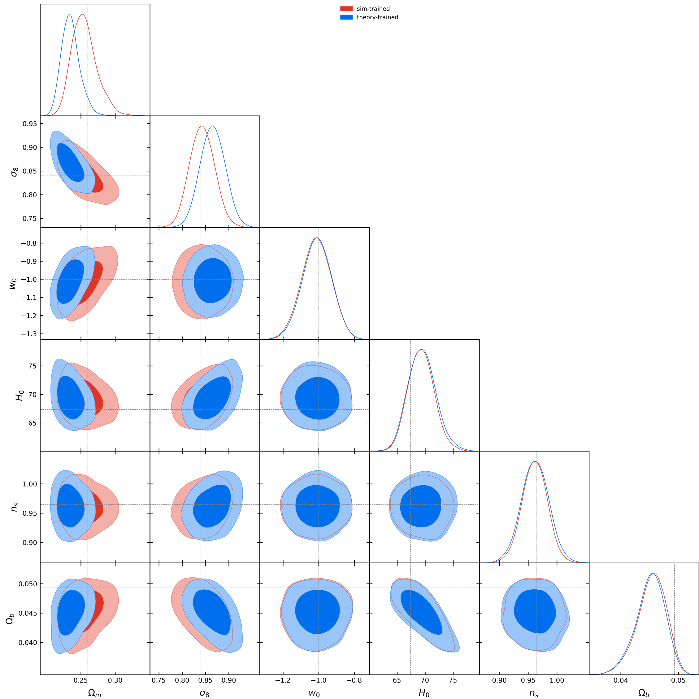
L1 NPE contours [bnt4]: sim vs theory, theta30, cut=aminm0p003_amaxp0p0009
