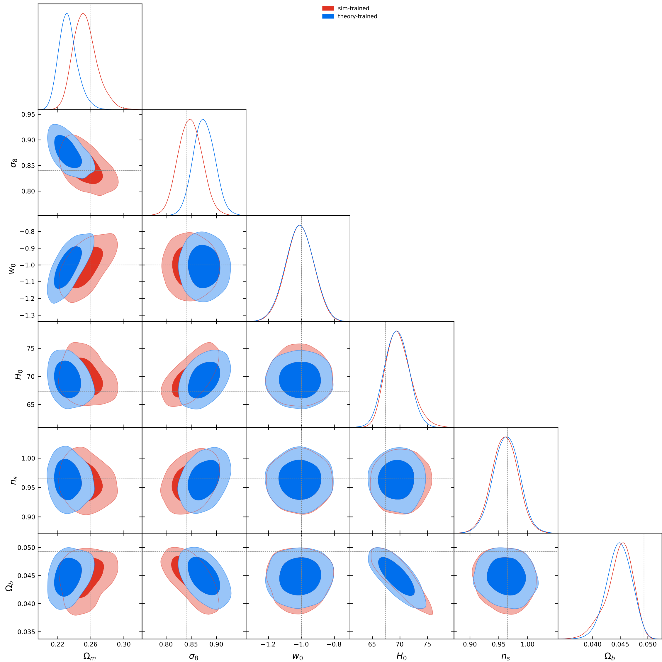
L1 NPE contours [bnt4]: sim vs theory, theta30, cut=full
