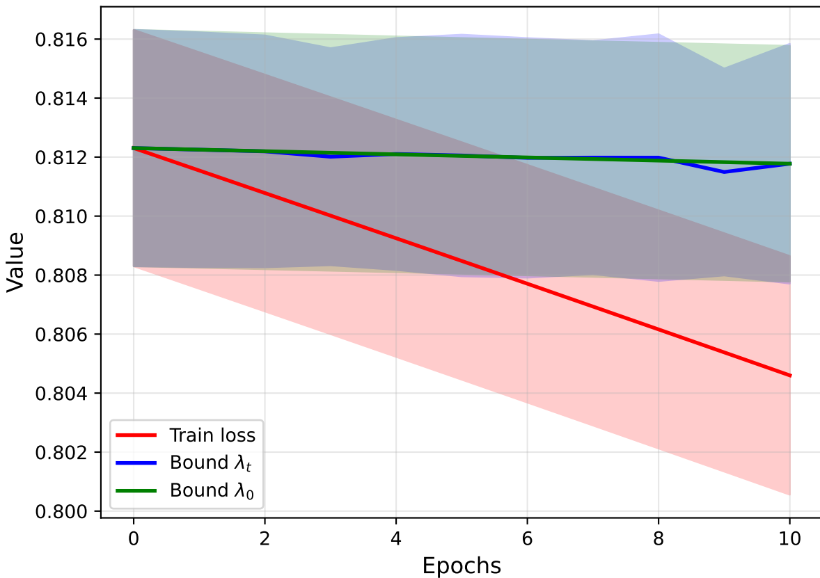
Hidden Size: 1000
