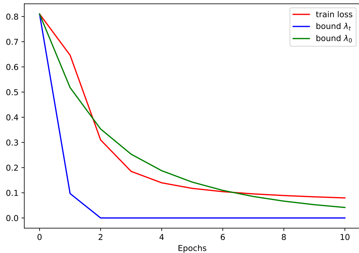
Hidden channel size : 100
