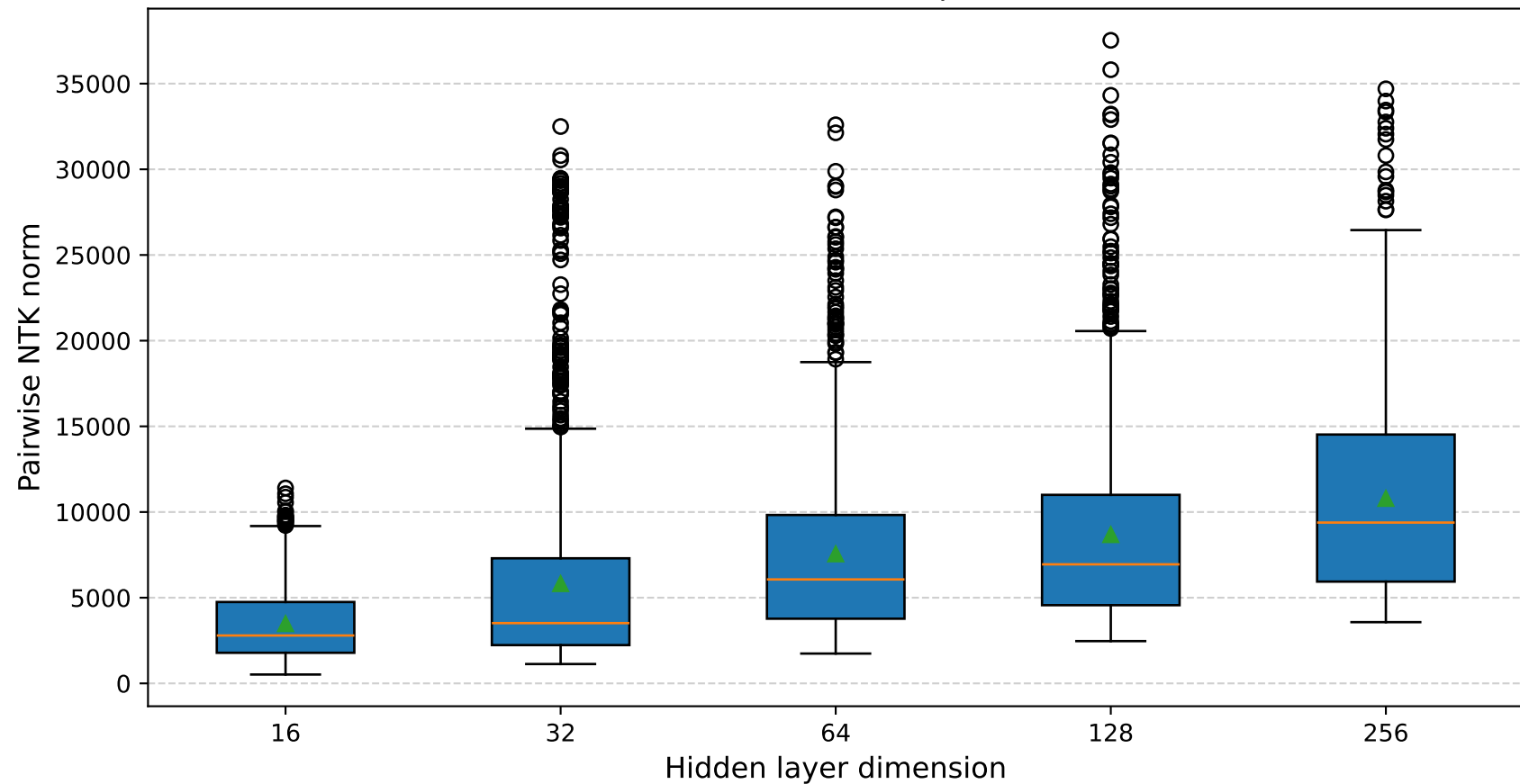
Distribution of Pairwise NTK Norms per Hidden Dimension
