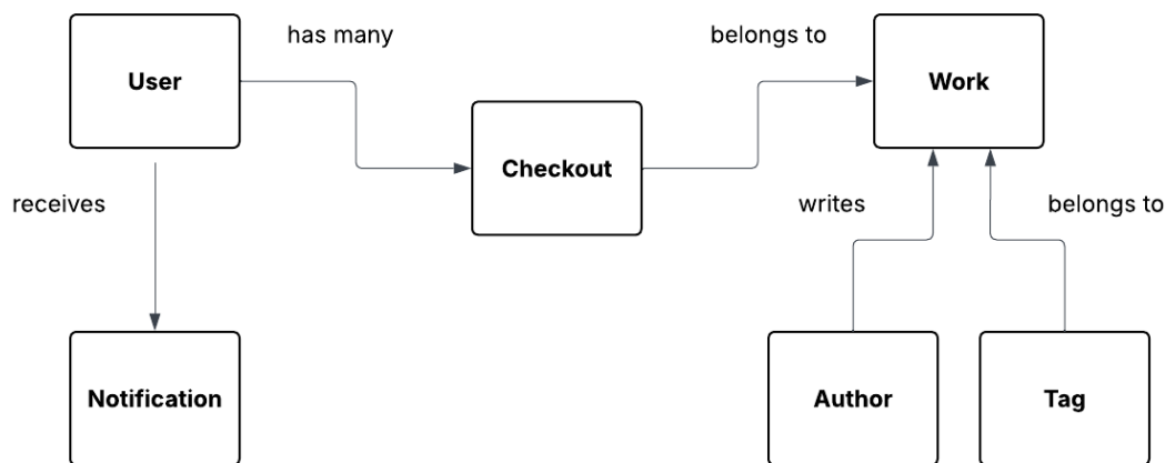
Figure 1: Simplified Class Diagram
