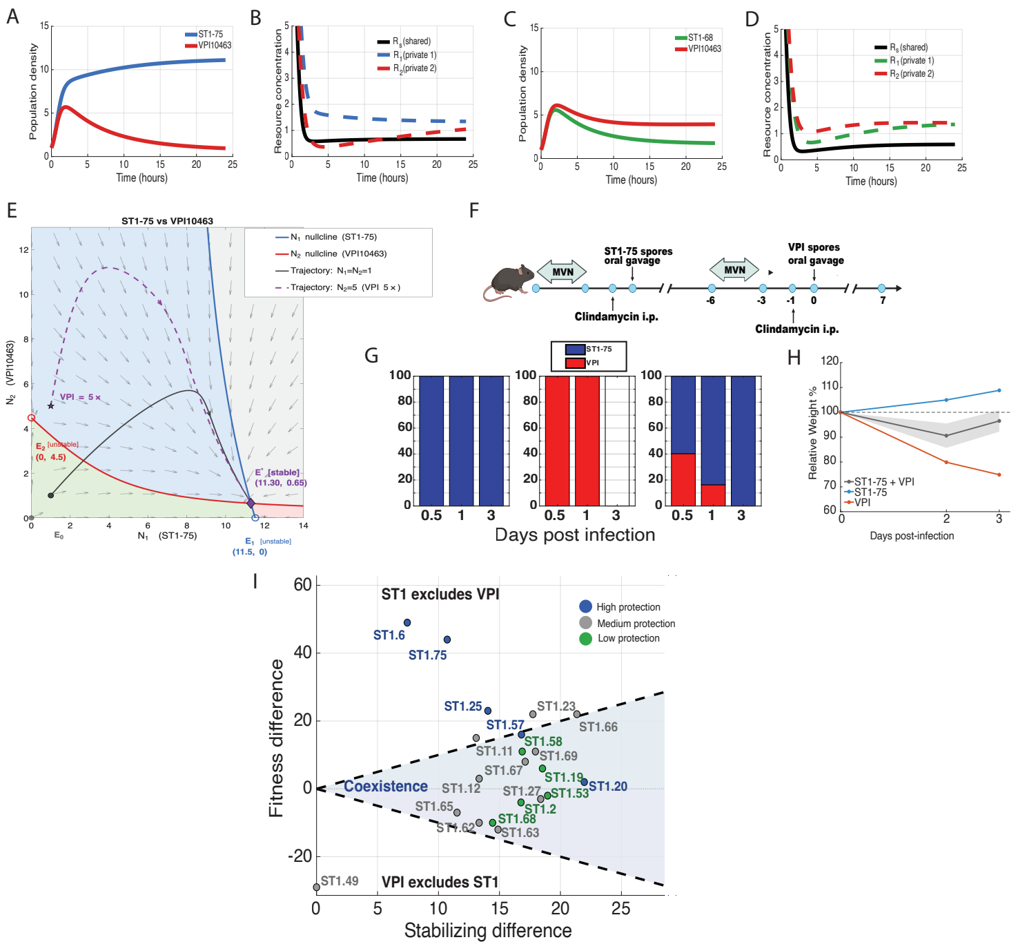
Figure 7: (A–B) Consumer resource model of competition between ST1.75 and VPI10463 strains grown on shared and private resources. (A) Population density dynamics over time (hours) for each strain. (B) Corresponding resource concentration dynamics, showing shared resource ( R_0 ) and private resources ( R_1 and R_2 ) for each strain. (C) Population density over time for each strain ST1.68 and VPI10463. (D) Resource concentration dynamics for shared and private resources, as in (B). (E) Phase-plane analysis of competition between ST1.75 and VPI10463. Solid blue and red lines indicate the N_1 (ST1.75) and N_2 (VPI10463) nullclines, respectively. Background shading indicates regions where only ST1.75 grows (blue), only VPI10463 grows (red), both strains grow (green), or neither grows (gray). Gray arrows indicate the vector field. Solid dark gray and dashed purple lines show representative trajectories initiated at N_1 = N_2 = 1 and N_1 = 1, N_2 = 5 (VPI 5 \times ), respectively. Open circles mark the single-strain equilibria E_1 (ST1.75 alone; unstable) and E_2 (VPI10463 alone; unstable). The filled purple diamond marks the stable coexistence equilibrium E^* with coordinates indicated. (F) Experimental timeline for mouse infection model. Mice were pretreated with clindamycin (i.p.), followed by oral gavage of ST1-75 spores, then a second clindamycin dose. MVN (mock vehicle or treatment) was administered at indicated timepoints. VPI spores were administered by oral gavage at day -1 relative to the final timepoint. (G) Stacked bar plots showing the proportion of mice colonized by ST1.75 (blue) vs. VPI (red) at 0.5, 1, and 3 days post-infection across three experimental conditions (left to right panels). (H) Relative weight (%) of mice colonized with ST1.75 + VPI (blue) vs. VPI alone (orange) over 3 days post-infection. Shaded region indicates the normal weight range. (I) Ecological coexistence analysis of multiple ST1 isolates plotted by stabilizing difference (x-axis) vs. fitness difference (y-axis). Dots are colored by protection level (dark blue = high, gray = medium, green = low). Regions of ST1 exclusion of VPI, coexistence, and VPI exclusion of ST1 are indicated. Dashed lines demarcate predicted coexistence boundaries based on modern coexistence theory.
