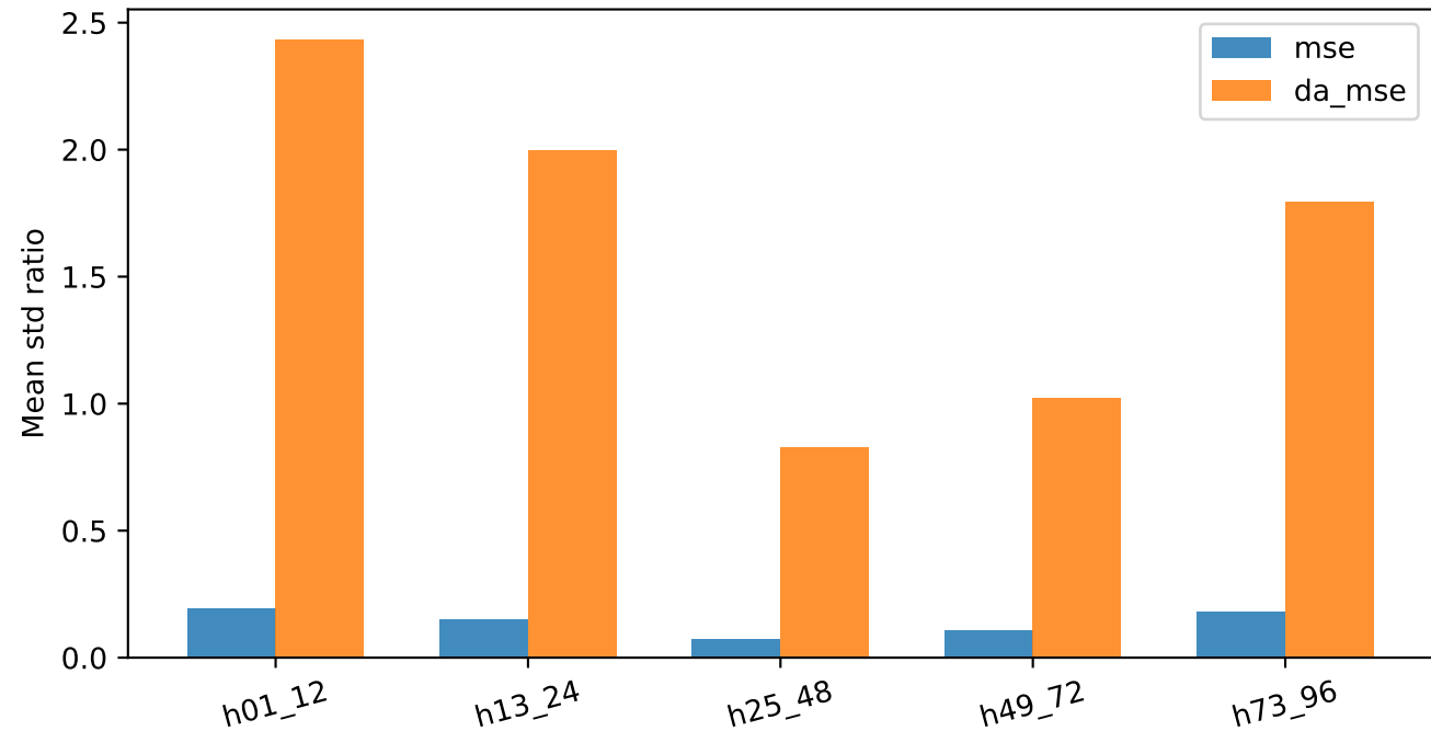
Horizon-wise variance recovery
