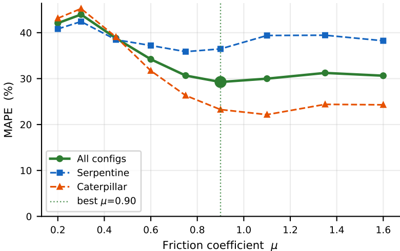
Sim-to-Real MAPE vs. Contact Friction (Plywood Surface)
