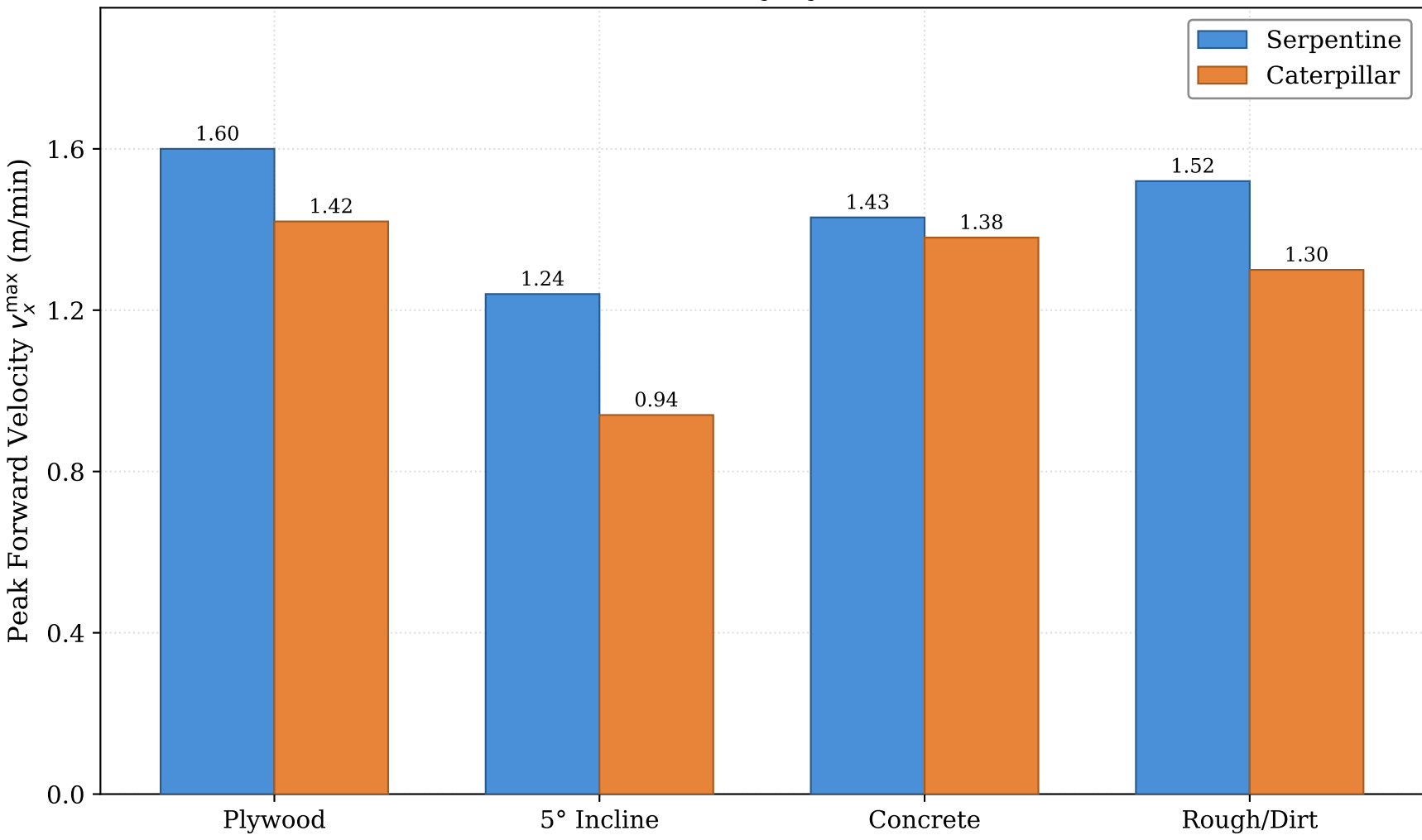
Peak Forward Velocity by Gait and Surface
