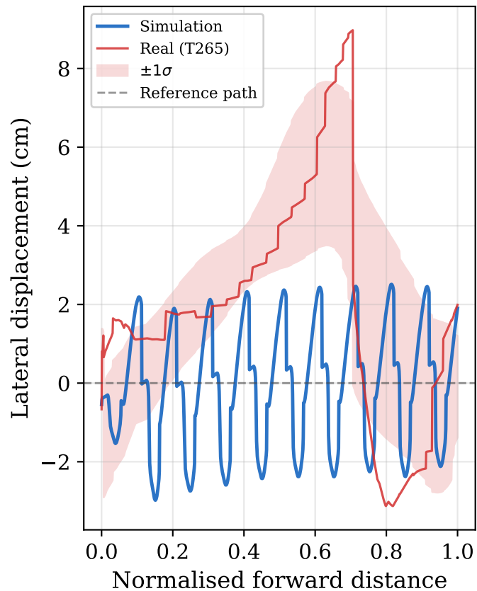
Lateral displacement, 10 cycles
