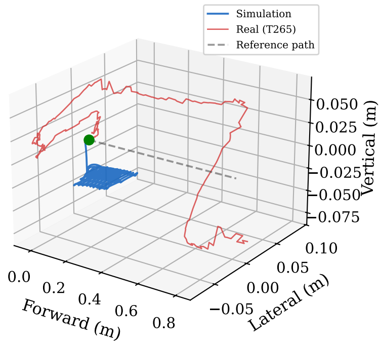
3-D head trajectory, serpentine A_y = A_z = 0.6 , f = 3.0 Hz
