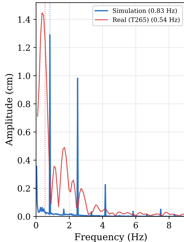
FFT of lateral oscillation
