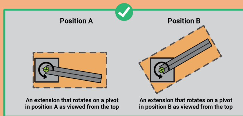
Figure 12-6: Expansion Limit – Rotating Extension
