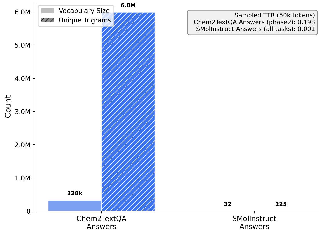
(A) Answer Lexical Diversity
