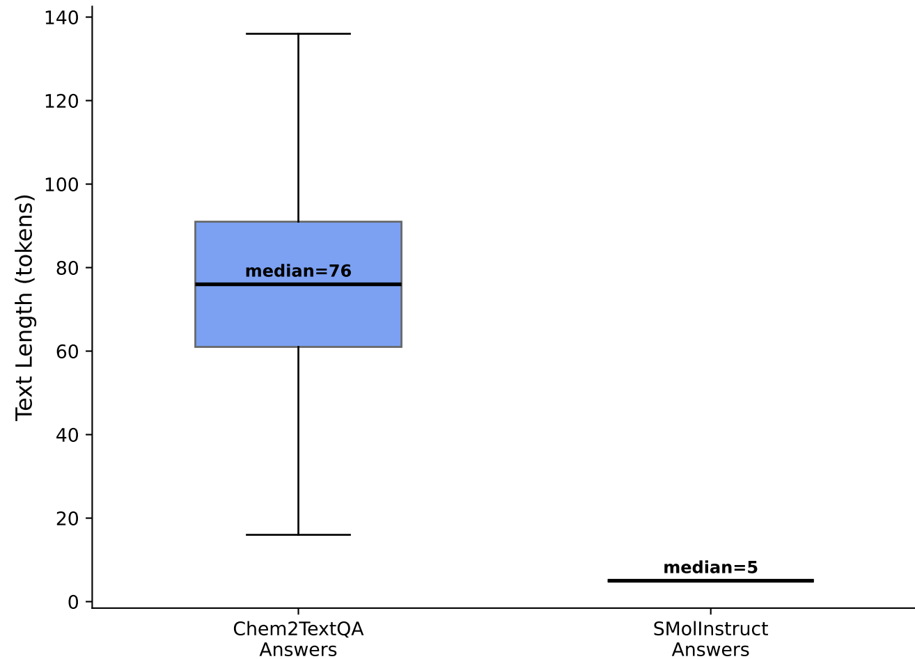
(B) Answer Text Length Distribution
