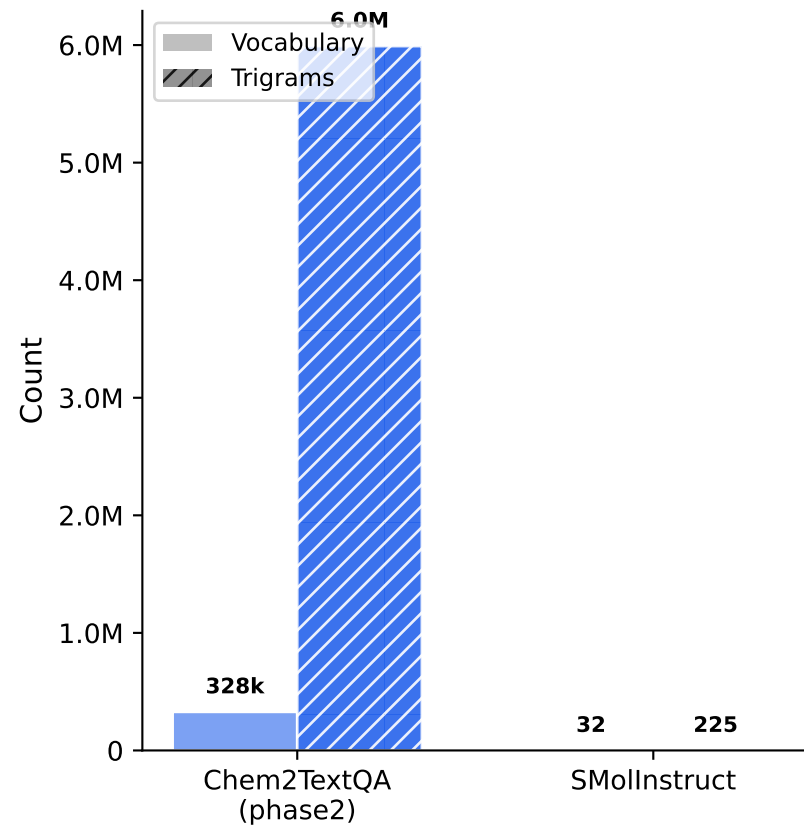
(A) Lexical Diversity
