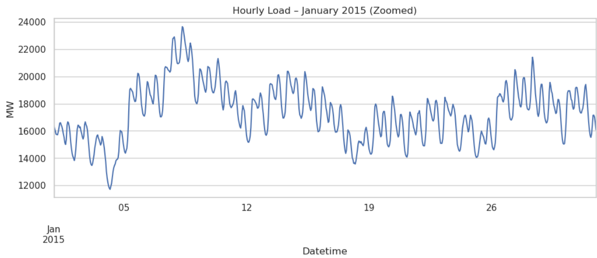
Figure 2: Hourly Electricity Load – January 2015; MW – MegaWatt
