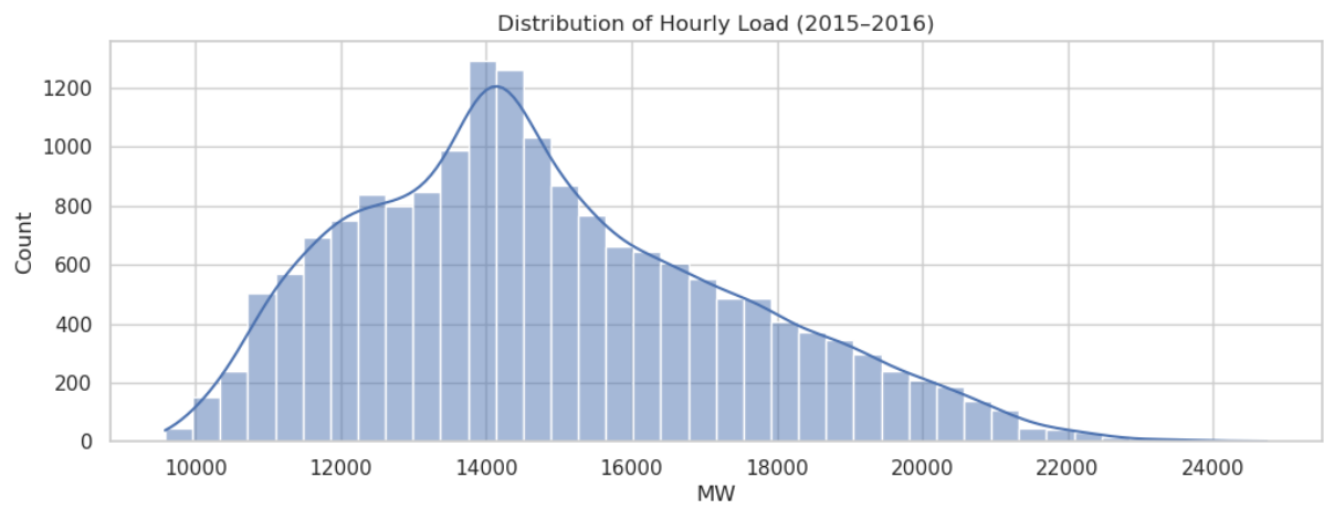
Figure 6: Hourly Load Frequency Distribution (2015 – 2016); MW – MegaWatt
