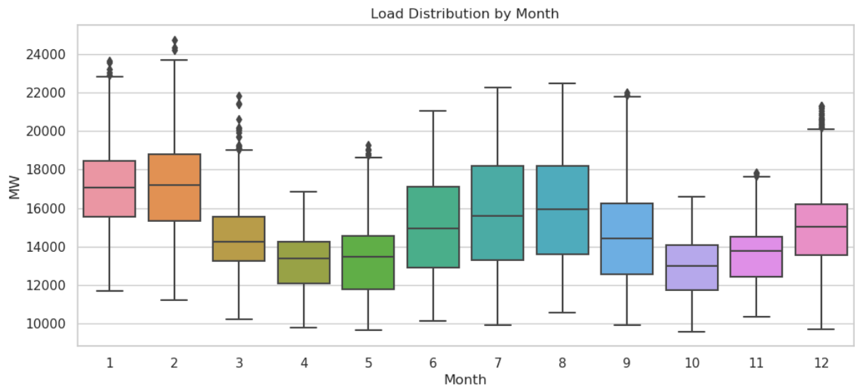
Figure 7: Box-Plot showing Monthly Load Frequency Distribution (2015 – 2016); MW – MegaWatt
