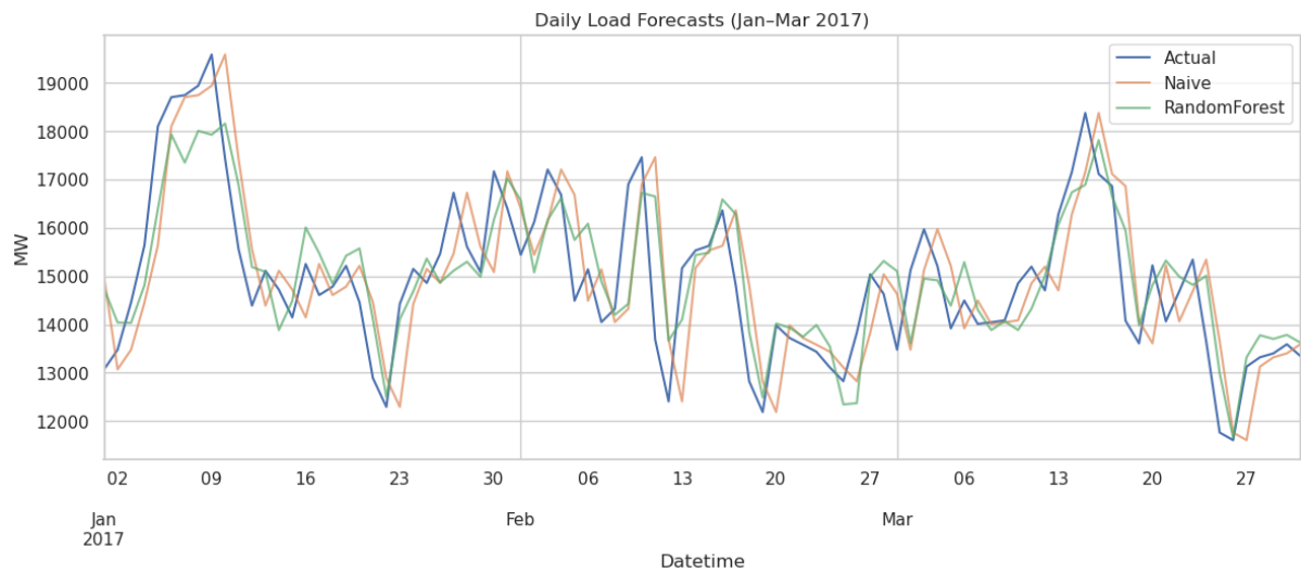
Figure 10: Daily Load Forecasts (Jan – Mar 2017) using Random and Baseline models; MW – MegaWatt
