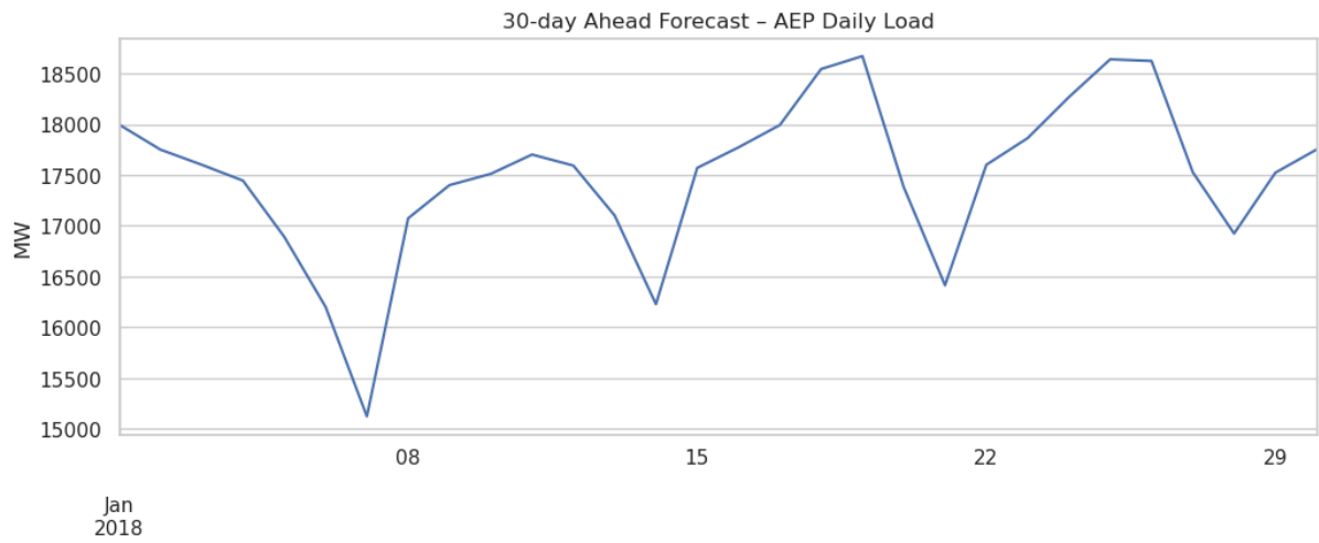
Figure 11: Furture prediction and forecast (30 days window) using Random Forest models; MW – MegaWatt
