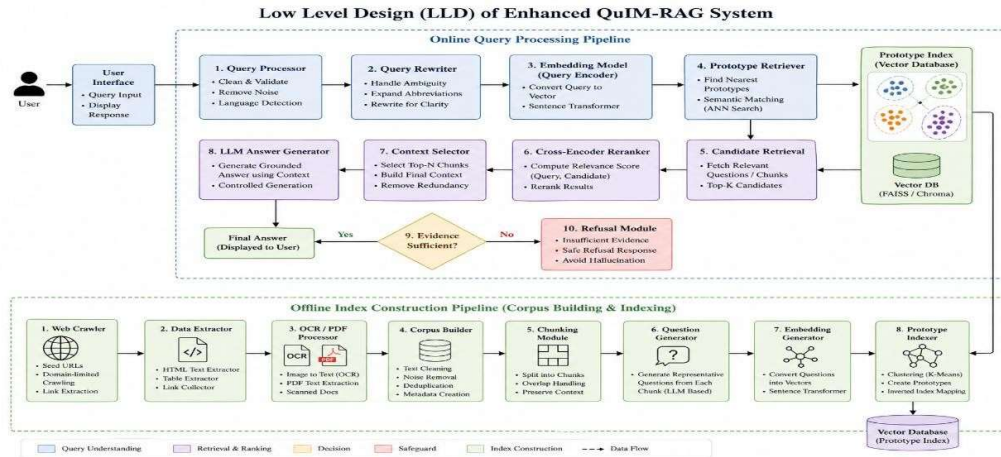
Fig 4.4 Low Level Design
