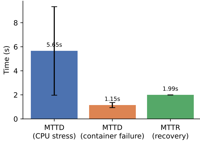
Fig. 9. Mean time to detect (MTTD) a CPU-stress event, MTTD for a killed container, and mean time to recover (MTTR) after restart, with error bars (one standard deviation), computed from the same raw detection/recovery times reported in Section VI. Binary failure (container killed) is detected roughly 5\times faster than gradual CPU saturation, since a scrape either observes the target down or it doesn’t, while a saturation threshold must be crossed by an accumulating signal.
