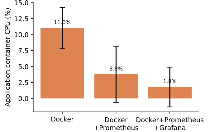
Fig. 5. Application container CPU utilization across the three monitoring cases (Table V, column 1). CPU% falls as more monitoring containers are added — the counter-intuitive result discussed under RQ3.
