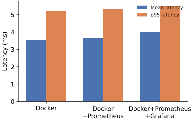
Fig. 7. Mean and p95 request latency across the three monitoring cases (Table V, columns 3-4). Both rise slightly as monitoring is added, consistent with the throughput drop and the host-contention explanation in Section VI.
