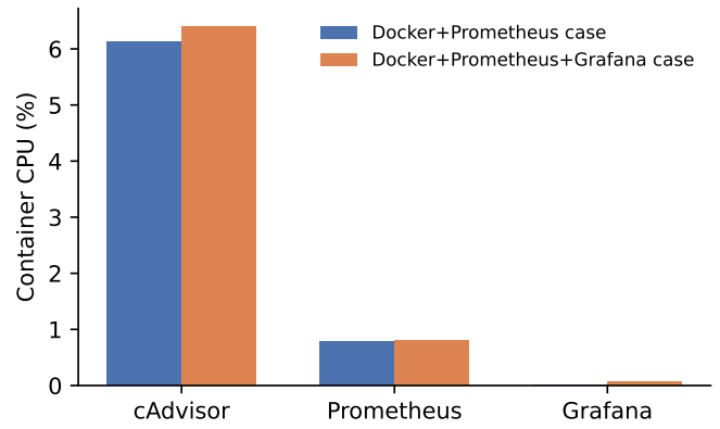
Fig. 10. Monitoring stack containers' own CPU draw (Table VI). cAdvisor dominates the monitoring stack's own overhead at \approx 6\% CPU in both cases; Prometheus and Grafana are comparatively cheap ( <1\% each). This is the overhead the monitoring tooling itself pays, separate from the host-contention effect on the application shown in Fig. 5.
