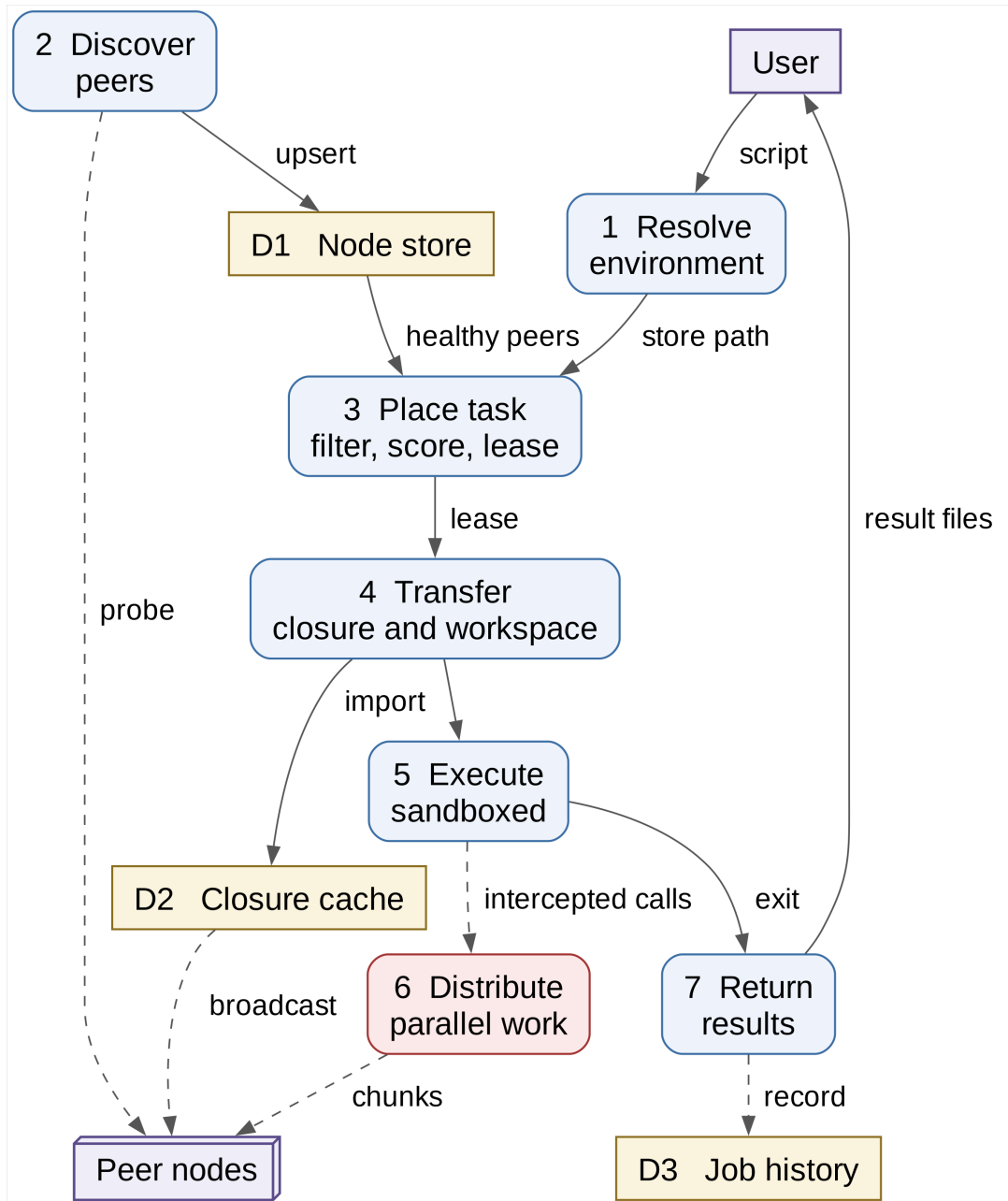
Figure 3.3: Level 1 DFD — seven processes over three data stores.
