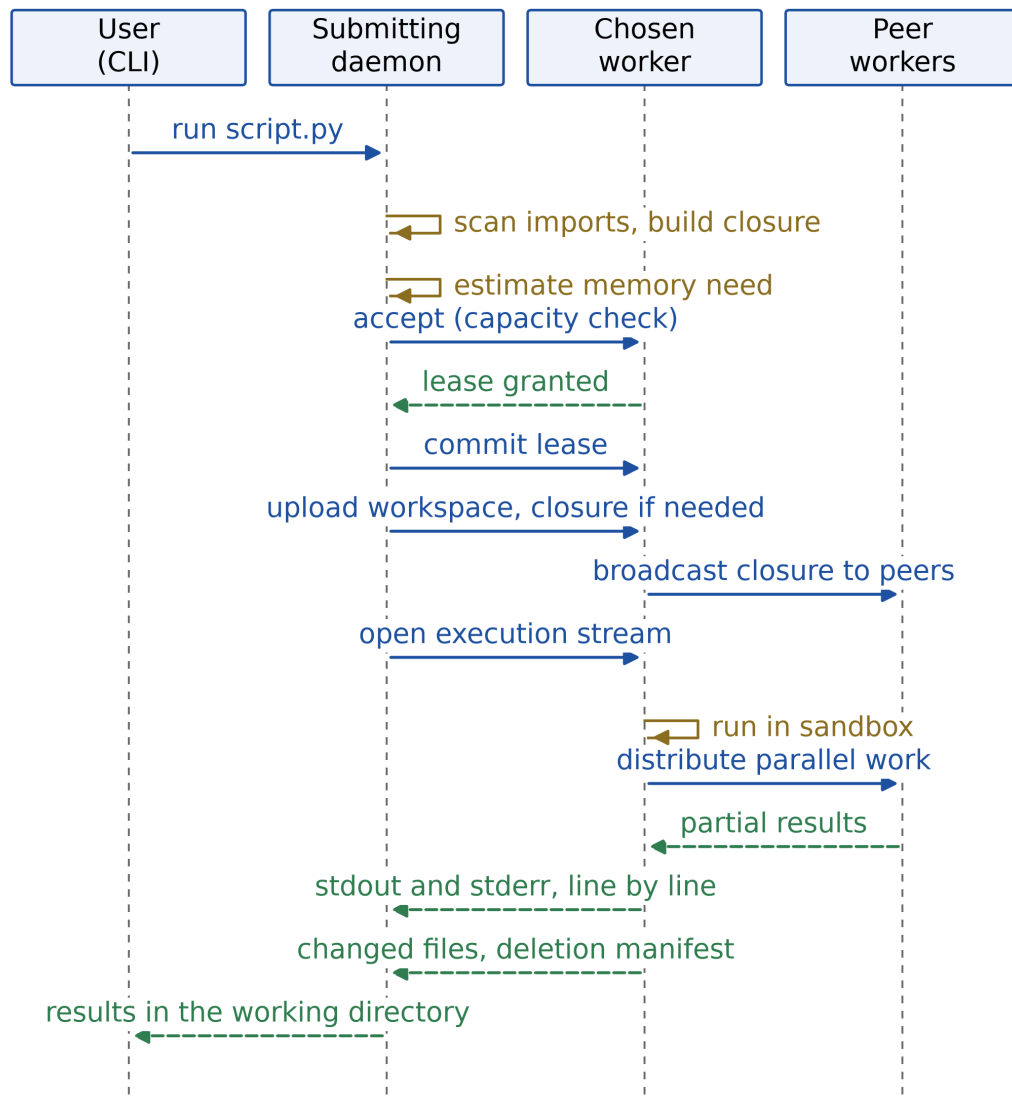
Figure 3.5: End-to-end execution of one job.
