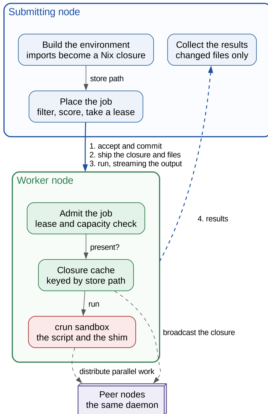
Figure 3.1: PipedPeer system design. The submitting side builds the environment and places the job; the worker admits it, caches the closure and runs it sandboxed. Both roles are the same binary.
