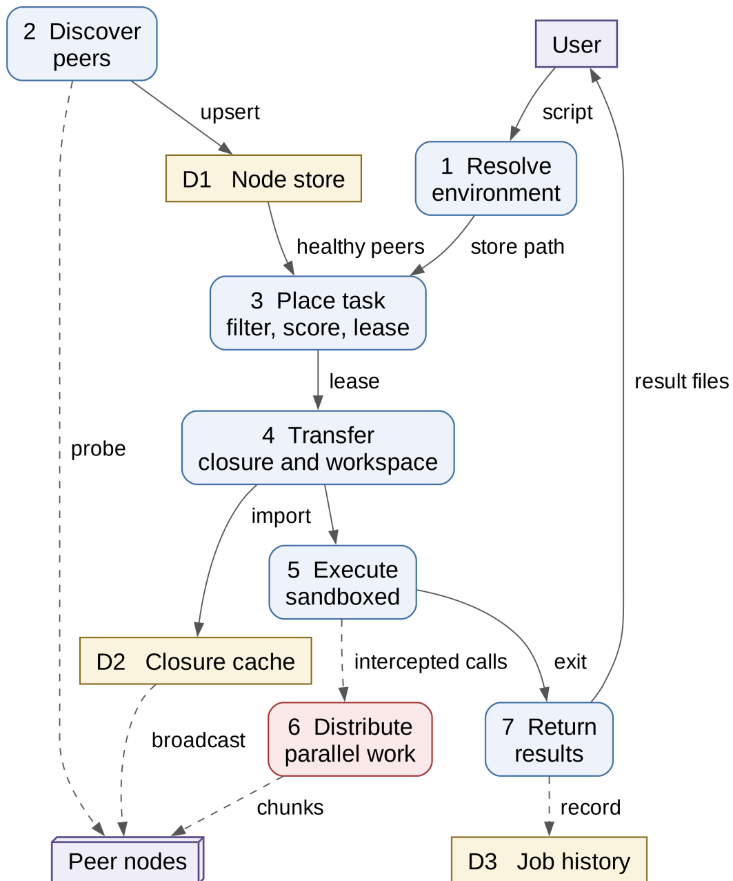
Figure 3.3: Level 1 DFD — seven processes over three data stores.
