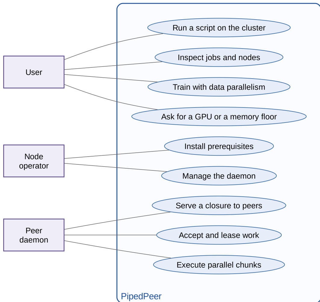
Figure 3.4: Use cases. A peer daemon is an actor in its own right, because every node serves closures and executes chunks for others.
