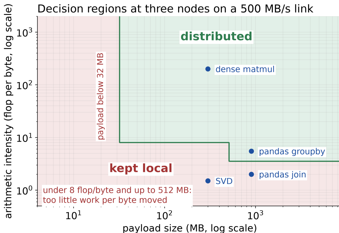
Figure 4.9: Decision regions from Equation 4.2. Dense matrix multiplication sits in the distributed region on paper but is held local by a separately calibrated model, because local BLAS beats the transport.
