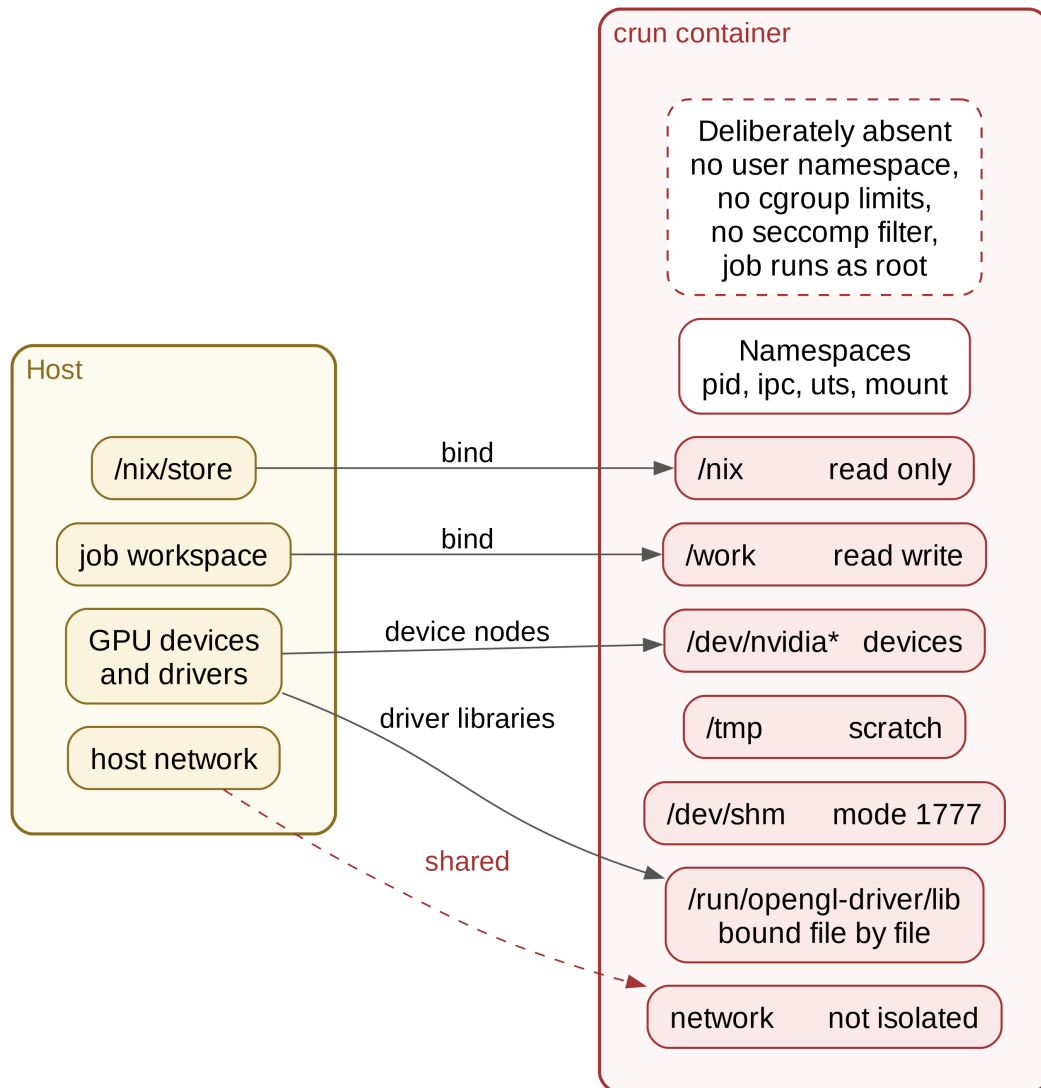
Figure 4.5: What the job can and cannot see. The absences are as deliberate as the mounts. Shared memory is mounted world-writable because Python’s multiprocessing requires it, and the driver libraries are bound file by file so that the host C library cannot shadow the closure’s.
