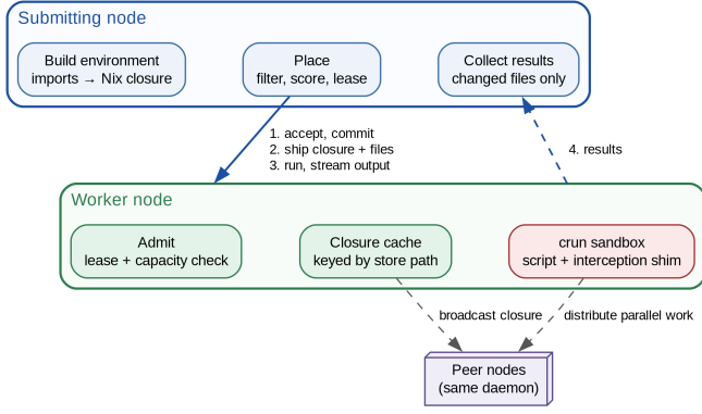
Fig. 1: System design. The submitting side builds the environment and places the job; the worker admits it, caches the closure and runs it sandboxed. Both roles are the same binary.
