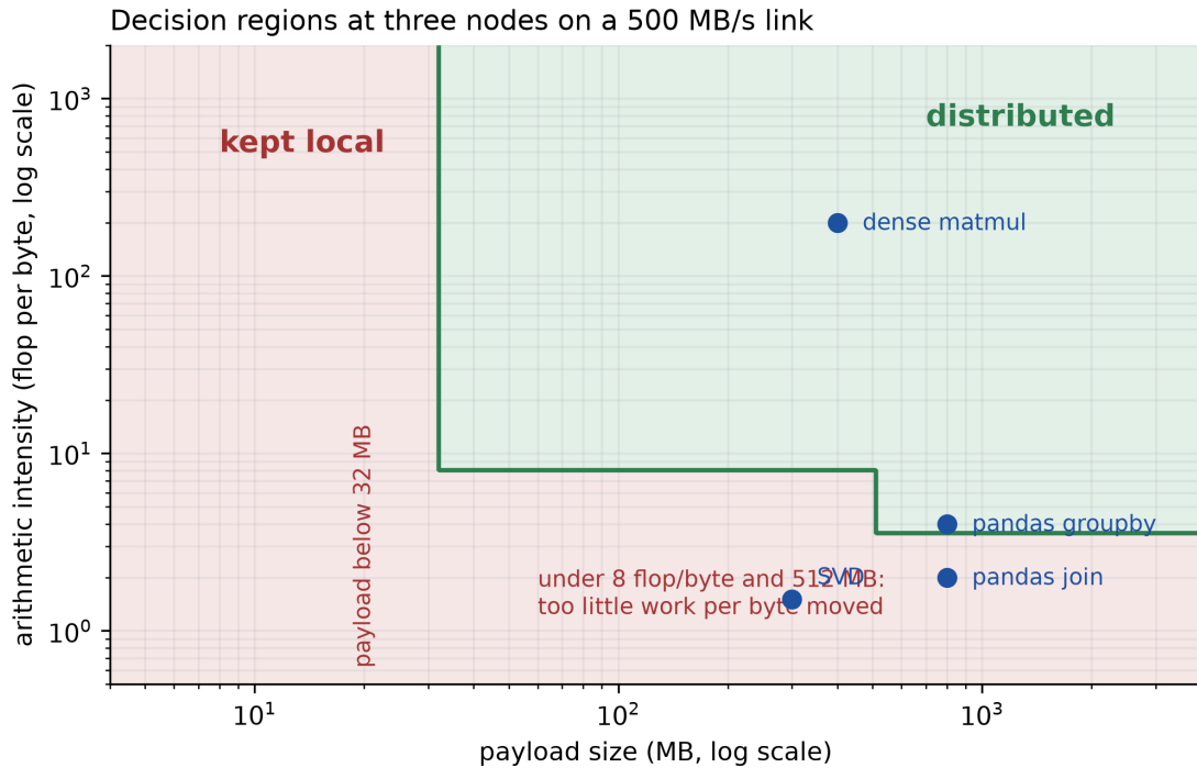
Figure 4.9: Decision regions from Equation 4.2. Dense matrix multiplication sits in the distributed region on paper but is held local by a separately calibrated model, because local BLAS beats the transport.
