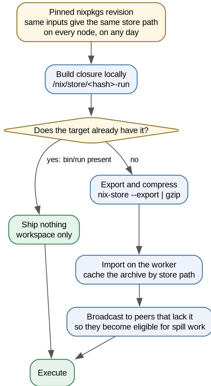
Figure 4.4: The store path is the cluster-wide cache key. Most submissions ship no environment at all.
