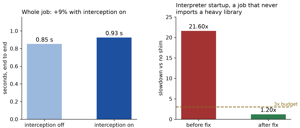
Figure 5.2: Left: cost over a whole job. Right: interpreter startup, before and after deferring library patching.
