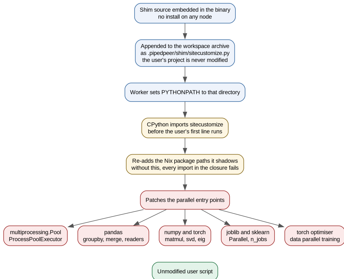
Figure 4.6: How the shim reaches the interpreter and what it replaces.
