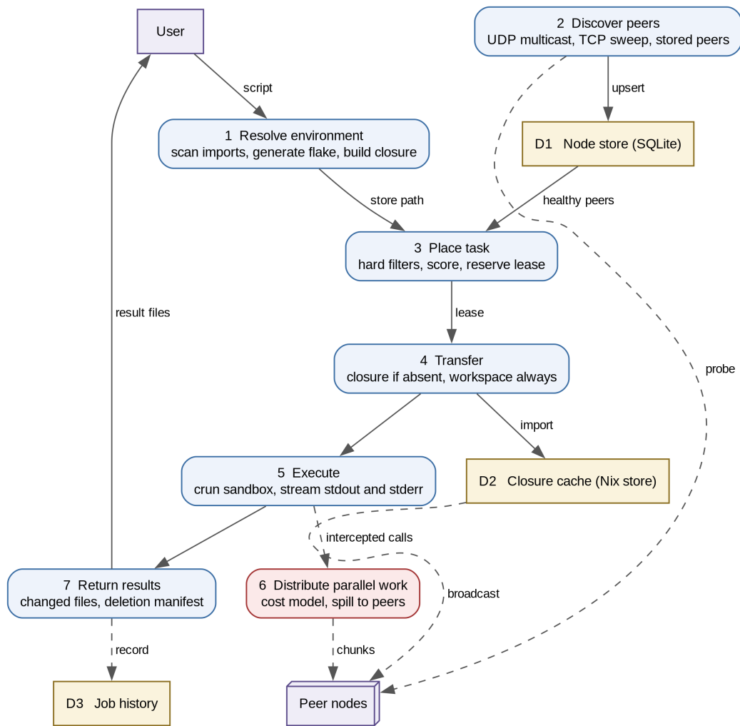
Figure 3.3: Level 1 DFD — seven processes over three data stores.
