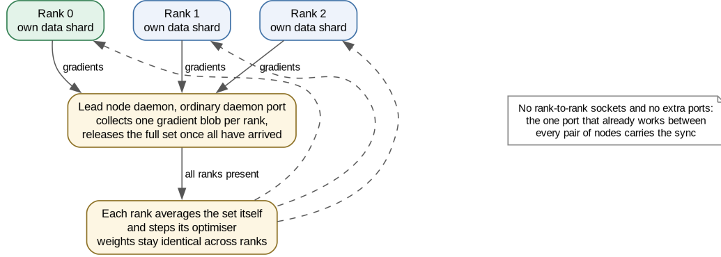
Figure 4.8: Gradient exchange over the daemon port.
