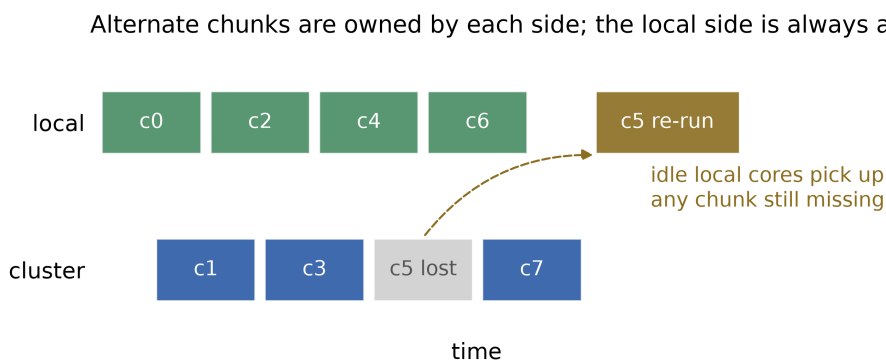
Figure 4.10: Racing local and remote work. The local side is always able to finish alone, which is what makes the guarantee unconditional.
