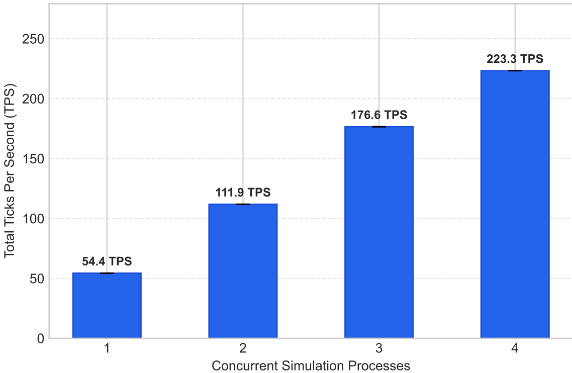
Total Aggregate Simulation Throughput vs Concurrency
