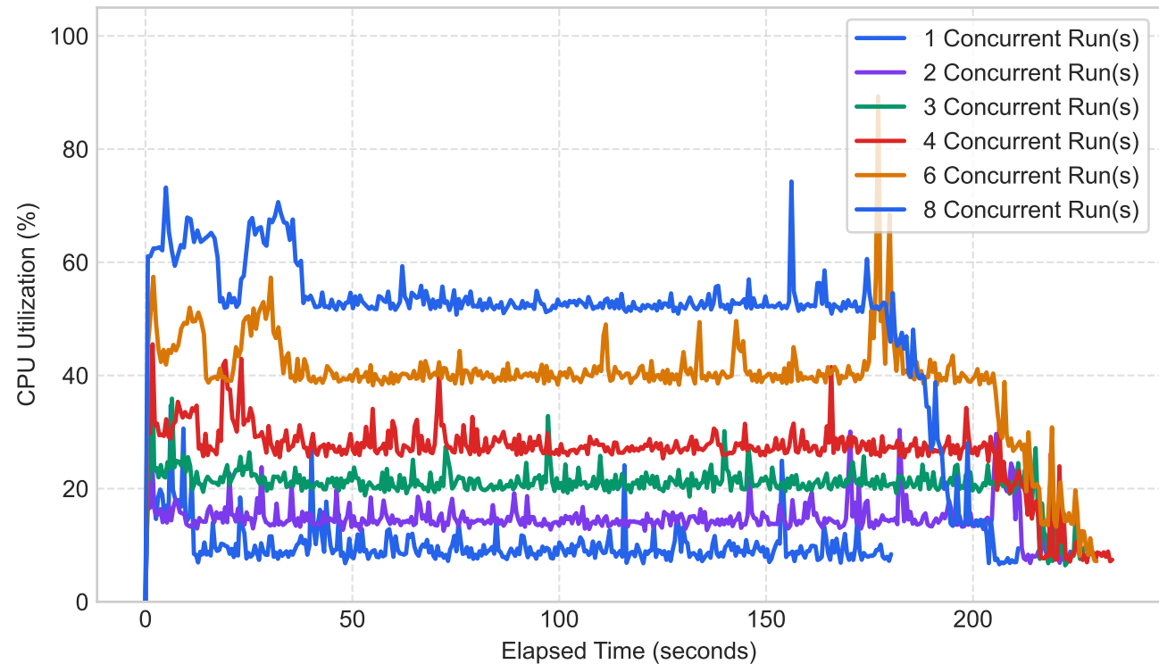
System CPU Utilization Over Time
