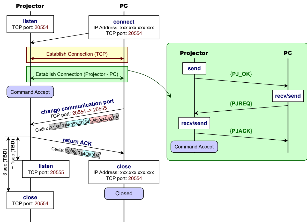
Figure2: Connection procedure at changing communication port (Example: 20554 → 20555)
