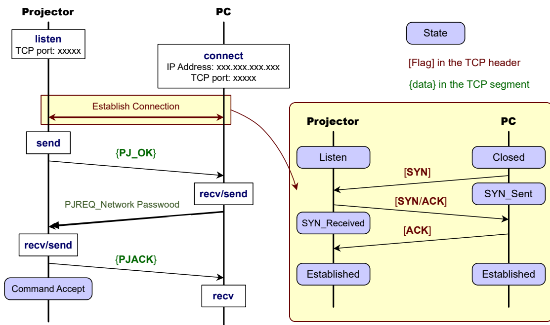
Figure1: Connection procedure at normal condition
