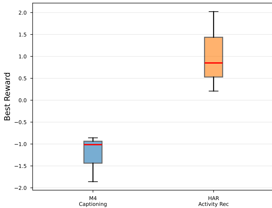
Reward Distribution
