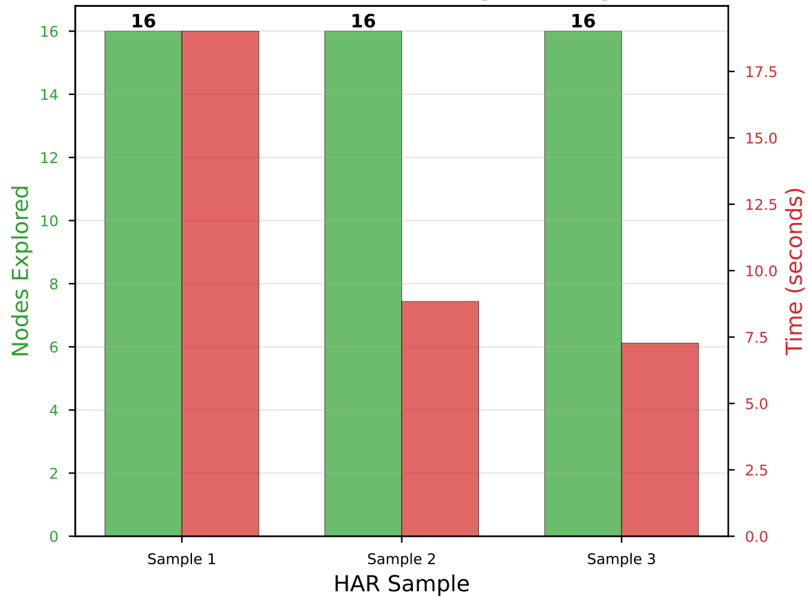
HAR: Nodes and Time per Sample
