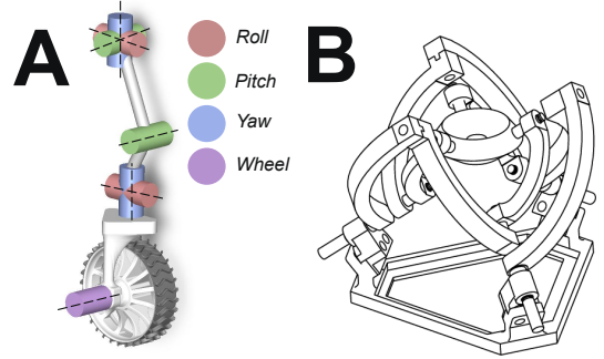
Figure 2: (A) 7-DOF wheeled leg architecture diagram with roll, pitch, and yaw joints color-coded. (B) 3-DOF parallel mechanism for reduced lower-leg inertia.
