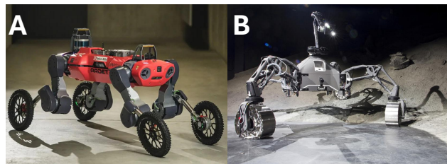
Figure 1: Examples of adaptive wheeled-legged rover platforms. (A) ANYmal with integrated mammalian wheeled legs, demonstrating transitions between walking and driving modes [10]. (B) SherpaTT in an arachnid-inspired configuration with articulated limbs for rough terrain navigation [11].
