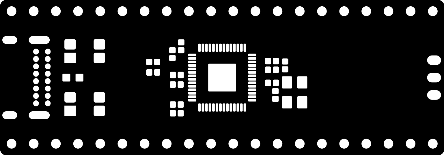
Top Solder (Scale 4:1)
