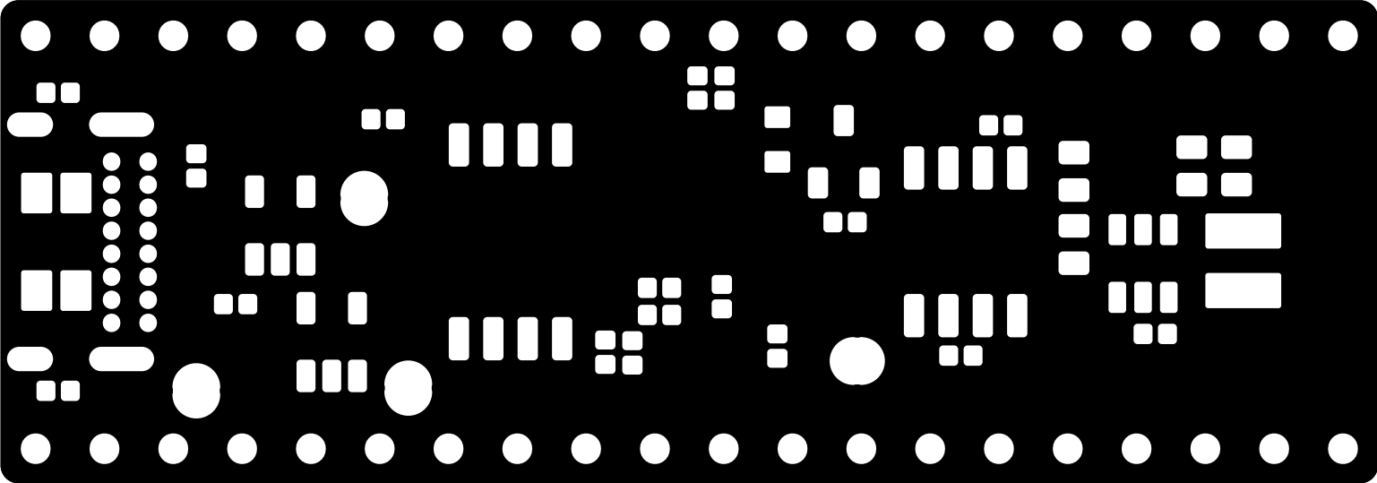
Bottom Solder (Scale 4:1)
