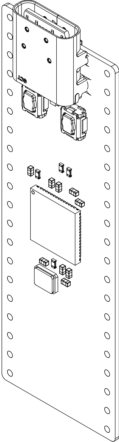
View from Top side (Scale 4:1)
