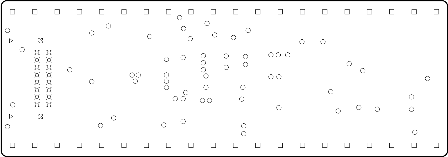
Drill Drawing View (Scale 4:1)
