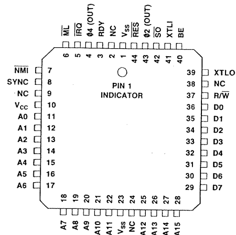
44-PIN PLCC
