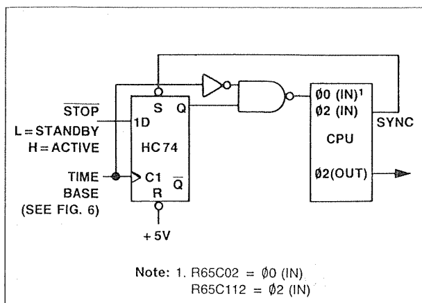
Figure 8. Stopping the Clock (Standby Mode) Circuit
