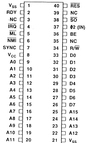
40-PIN DIP
