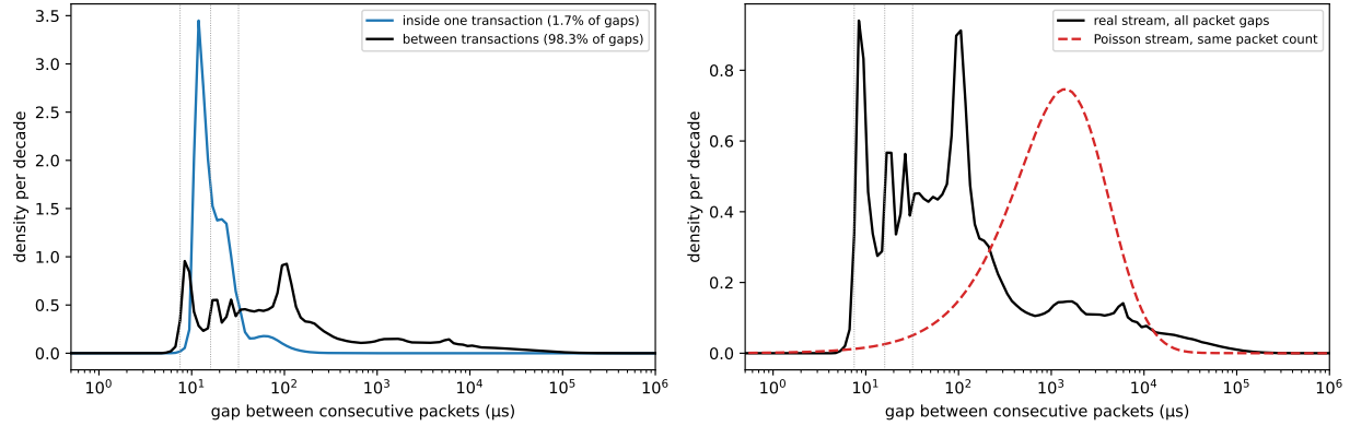
Figure 4. Packet interarrival gaps, pooled over the corpus, density per decade on a logarithmic gap axis; dotted lines at 7.5 , 16 and 32 \mu\text{s} . Left: gaps between two packets of the same transaction ( 5.6 \times 10^7 ) against gaps between packets of different transactions ( 3.24 \times 10^9 ). Each curve is normalised to its own total, so heights compare shapes, not counts (the blue gaps are 1.7% of all gaps, the black 98.3%). What it shows: the intra-transaction distribution is a single narrow peak at 12\text{--}16 \mu\text{s} with almost no mass below 10 \mu\text{s} and none below the floor — the pieces of one event are paced by the exchange at about 15 \mu\text{s} , slower than the closest that two packets of different events arrive, so the tightest gaps on the feed are never between pieces of the same event; the inter-transaction distribution has a sharp edge at the 7.5 \mu\text{s} floor, a broad plateau from the floor to about 30 \mu\text{s} , a second mode near 100 \mu\text{s} , and a long tail to seconds. Right: all packet gaps of the real stream (black; since 98.3% of gaps are between transactions this curve is the left panel's black curve with the blue one folded in) against the gaps of a Poisson stream with the same packet count over the same window (red, dashed), the distribution a receiver would face if the market's events were independent of one another at the observed rate. What it shows: the Poisson density is a single hump centred near 1 \text{ ms} with negligible mass below 100 \mu\text{s} ; the real density puts a third of its mass below 32 \mu\text{s} , with the floor edge and the 100 \mu\text{s} mode absent from the null. The two curves are not two versions of the same shape: the real feed is not a Poisson stream, and the region in which it differs is exactly the region of gaps shorter than an HFT service time. What follows: the edge at 7.5 \mu\text{s} is a property of the gateway — no two packets of any origin are published closer than that — and it sets where a queue first forms; everything between the floor and 32 \mu\text{s} is gaps between different transactions, so the queueing regime of an HFT receiver is populated by distinct matching events arriving within one service time of each other, not by fragments of one event; and the whole of that region is absent from a Poisson stream at the same rate, which is why the uniform null in Table 2 has no tail below 32 \mu\text{s} . The 100 \mu\text{s} mode is the characteristic spacing of successive transactions within a burst, the time scale on which the self-excitation of Table 6 acts.
