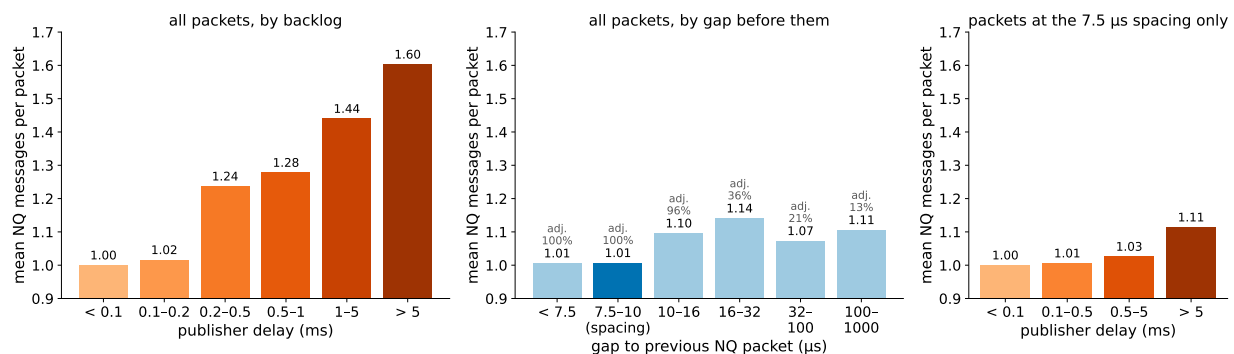
Figure 19. Tables 15–17 as bars: mean NQ messages per packet. Left: packets get bigger as the publisher falls further behind. Middle: packets sent at the publisher spacing, 7.5\text{--}10 \mu s after the previous NQ packet (dark blue), are single-message packets; the grey “adj.” figures are the share with no other order or trade packet of the channel between the two NQ packets, 100% at the spacing. Right: packets at the spacing stay single-message even when the publisher is more than 5 \text{ ms} behind. The publisher drains a backlog with more packets, not bigger ones.
