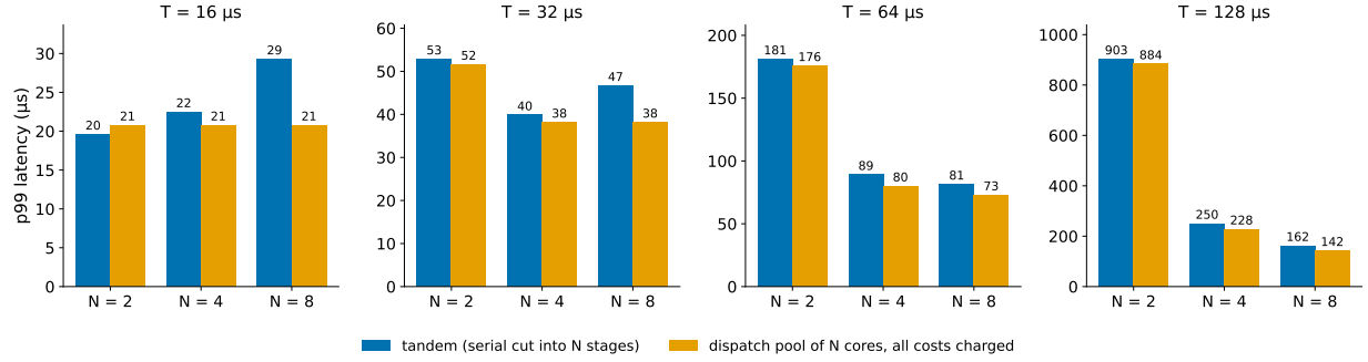
Figure 11. Table 9 as bars: p_{99} of a serial cut into N stages (blue) against a pool of N cores with the ingress hop, egress hop and resequencing charged (orange). At N = 2 the two are level; from N = 4 the pool is lower at every service time, and at 16 \mu s its p_{99} does not grow with N while the tandem's does.
