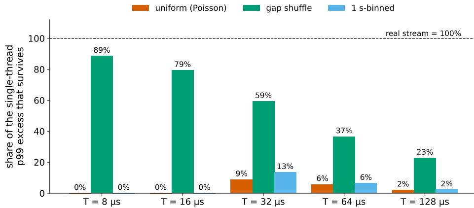
Figure 3. Table 3 as bars: the share of the single-thread p_{99} excess ( p_{99} - T ) that survives each null stream, the real stream being 100%. The gap shuffle (green), which keeps every gap and destroys their order, keeps most of the tail at 8\text{--}16\mu\text{s} and less as T grows: at short service times the tight gaps carry the tail, at long ones their arrangement into runs. The uniform and 1 s-binned streams keep almost none at any T .
