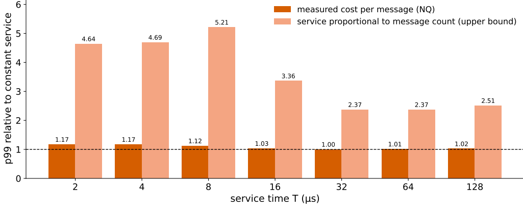
Figure 26. Table 25 as bars: p_{99} under service that grows with the message count, relative to constant service with the same mean. With the measured cost per message (vermillion) the tail is 12–17% larger at 8 \mu s and below and within 3% from 16 \mu s . The exaggerated model in which service is proportional to message count (light) bounds the effect from above.
