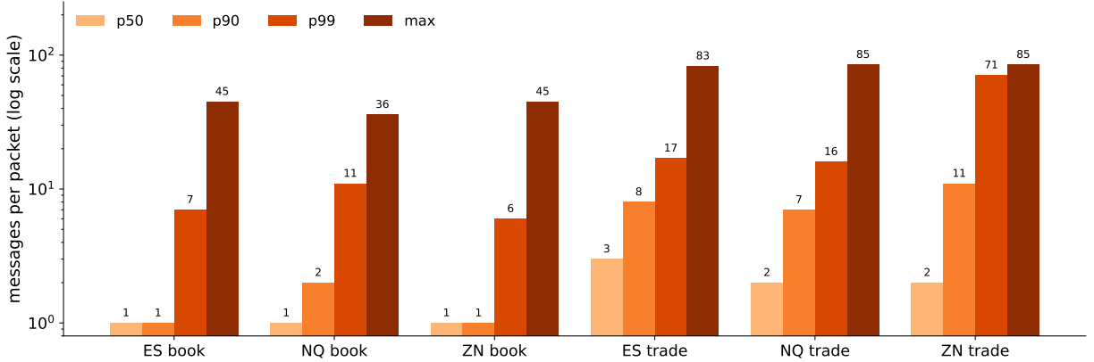
Figure 24. Table 23 as bars, log scale: messages per packet at the median, 90th and 99th percentile and the maximum, per live stream. Book streams carry one message in most packets and up to 45; trade streams carry more, and ZN trade reaches 71 at p_{99} .
