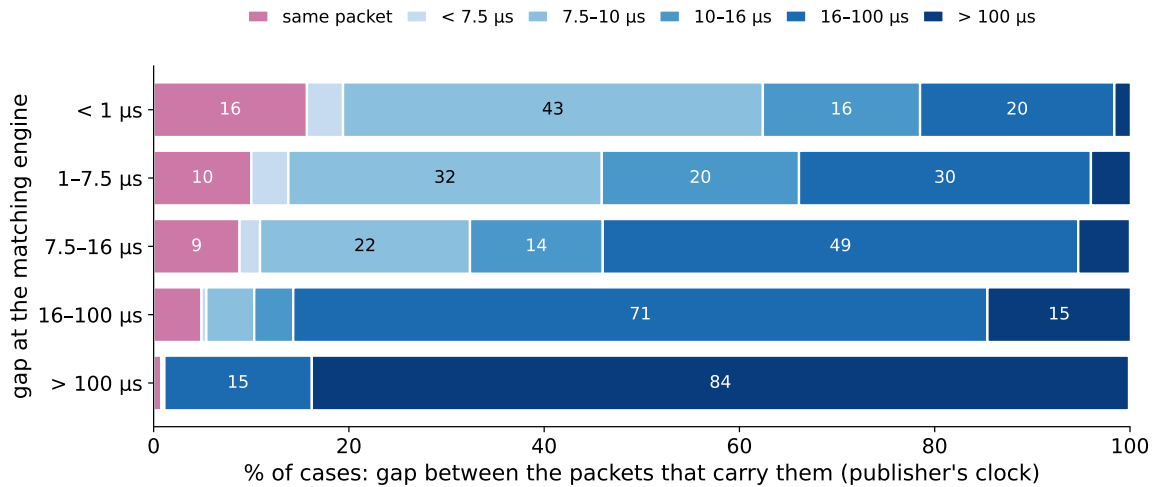
Figure 17. Table 13 as bars. Each bar is the set of consecutive transactions with the engine gap on the left, split by the gap between the packets that carry them; the numbers are percent of the bar. The top bar reads: when the engine processes a transaction less than 1 \mu s after the previous one, the two share a packet 16% of the time (pink) and otherwise arrive in separate packets, most often 7.5–10 \mu s apart (43%). Near-simultaneous at the engine becomes back to back at the publisher's spacing at the receiver.
