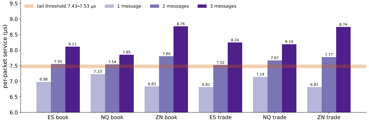
Figure 23. Table 22 as bars: per-packet service for one, two and three messages on each live stream, against the tail threshold (shaded band). A one-message packet is served below the threshold on every stream; a two-message packet is at or above it on every stream. Whether a packet can start a queue is decided by whether it carries more than one message.
