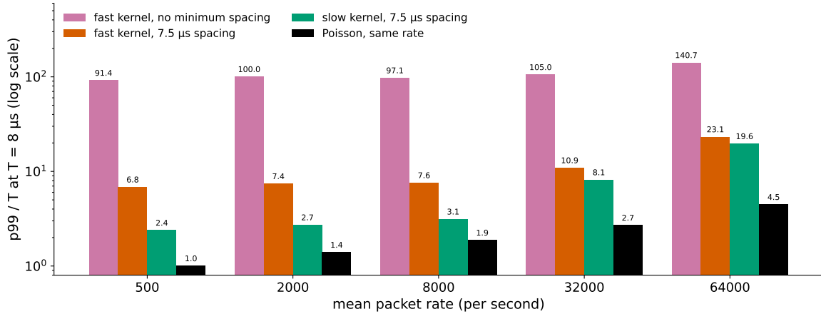
Figure 31. Table 30 as bars, log scale, for branching ratio 0.8: the normalised tail p_{99}/T at T = 8 \mu s on synthetic feeds, by packet rate. A fast kernel with no minimum spacing (pink) has a tail of about 100 times T ; adding a 7.5 \mu s minimum spacing (vermillion) cuts it more than tenfold; a slow kernel with the spacing (green) is lower still, 2 to 3 times T at low rates against 1 to 2 for the Poisson stream (black). What sets the tail at 8 \mu s is how many gaps sit at the minimum spacing, which the kernel and the spacing control and the branching ratio alone does not.
