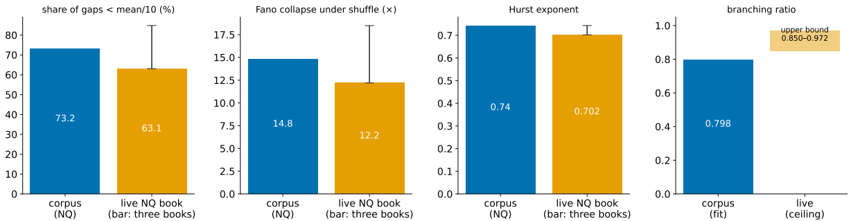
Figure 21. Table 21 as bars: the clustering statistics on the recorded corpus (blue) and on the live receiver’s NQ book stream (orange; whiskers span the three live book streams). The share of tiny gaps, the collapse of the Fano factor under shuffling and the Hurst exponent agree within the spread of the live streams. The corpus branching ratio lies below every upper bound the live streams give (shaded).
