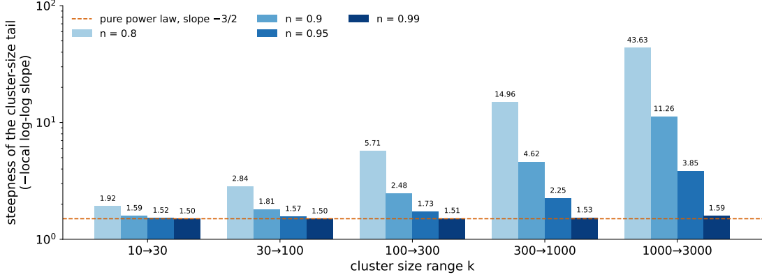
Figure 30. Table 29 as bars, log scale: how steeply the cluster-size distribution falls over successive size ranges, for four branching ratios. Near criticality ( n = 0.99 ) it keeps the power-law slope of 3/2 (dashed) over the whole range; at n = 0.8 it falls off exponentially beyond about 25, so very large clusters are rare.
